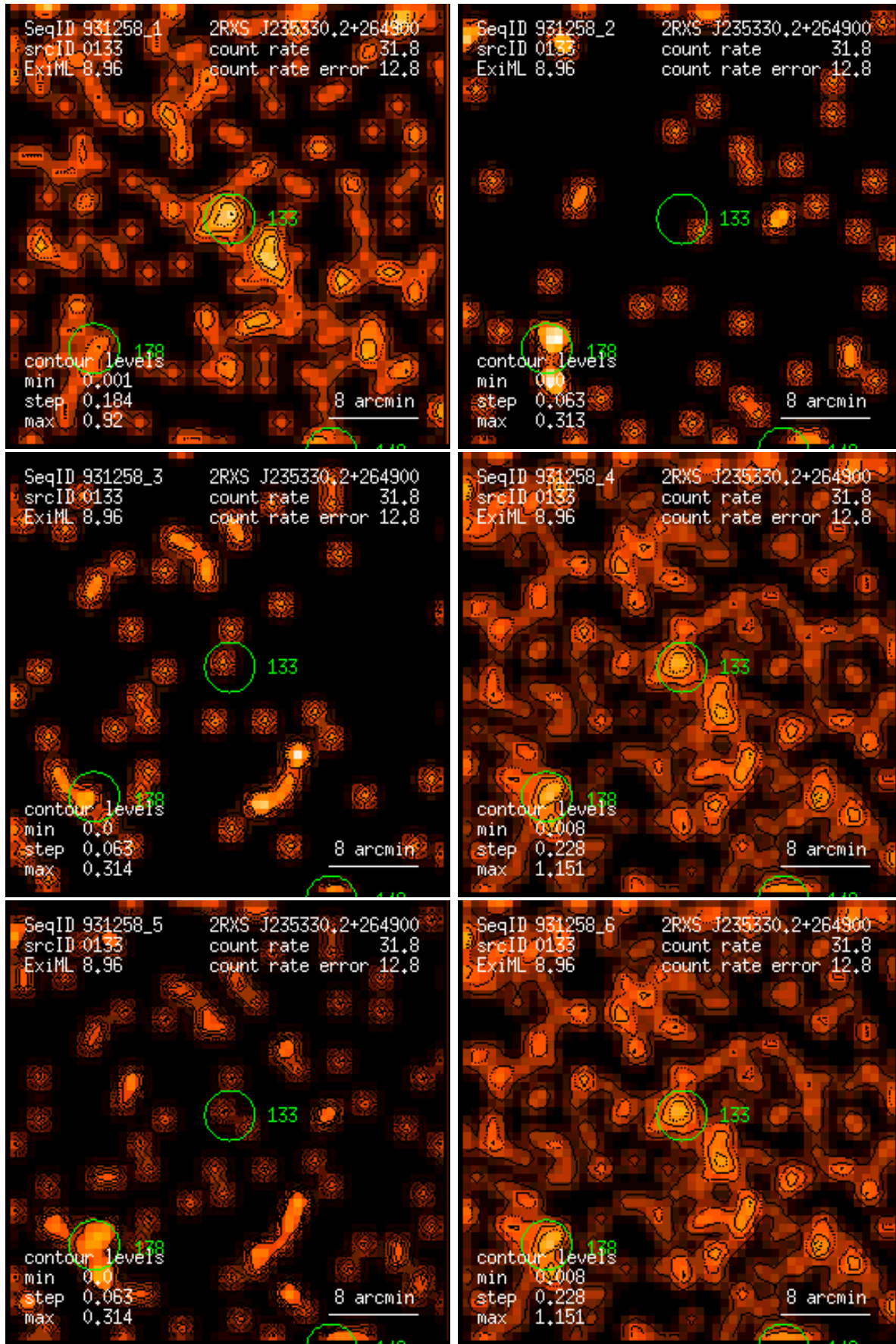
Figure 133: RASS 931258: detection 0133: band rate images, Gaussian filter: (1) PSPC channels 11 – 41, (2) 52 – 90, (3) 91 – 201, (4) 11 – 235, (5) 52 – 201, (6) 11 – 201. Broad band rates in counts/ks. Band rate contour levels in counts/ks/arcmin 2 .
