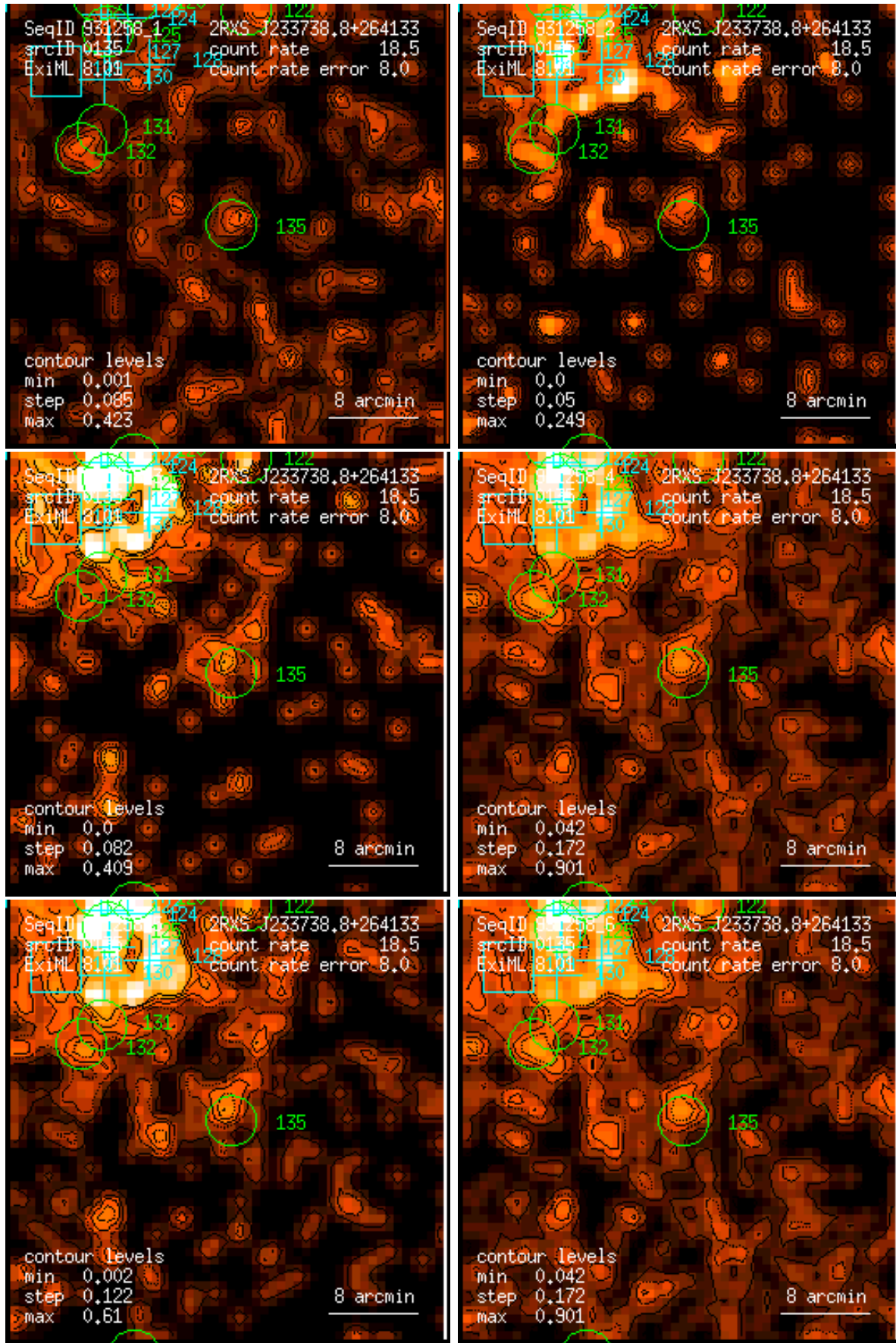
Figure 135: RASS 931258: detection 0135: band rate images, Gaussian filter: (1) PSPC channels 11 – 41, (2) 52 – 90, (3) 91 – 201, (4) 11 – 235, (5) 52 – 201, (6) 11 – 201. Broad band rates in counts/ks. Band rate contour levels in counts/ks/arcmin 2 .
