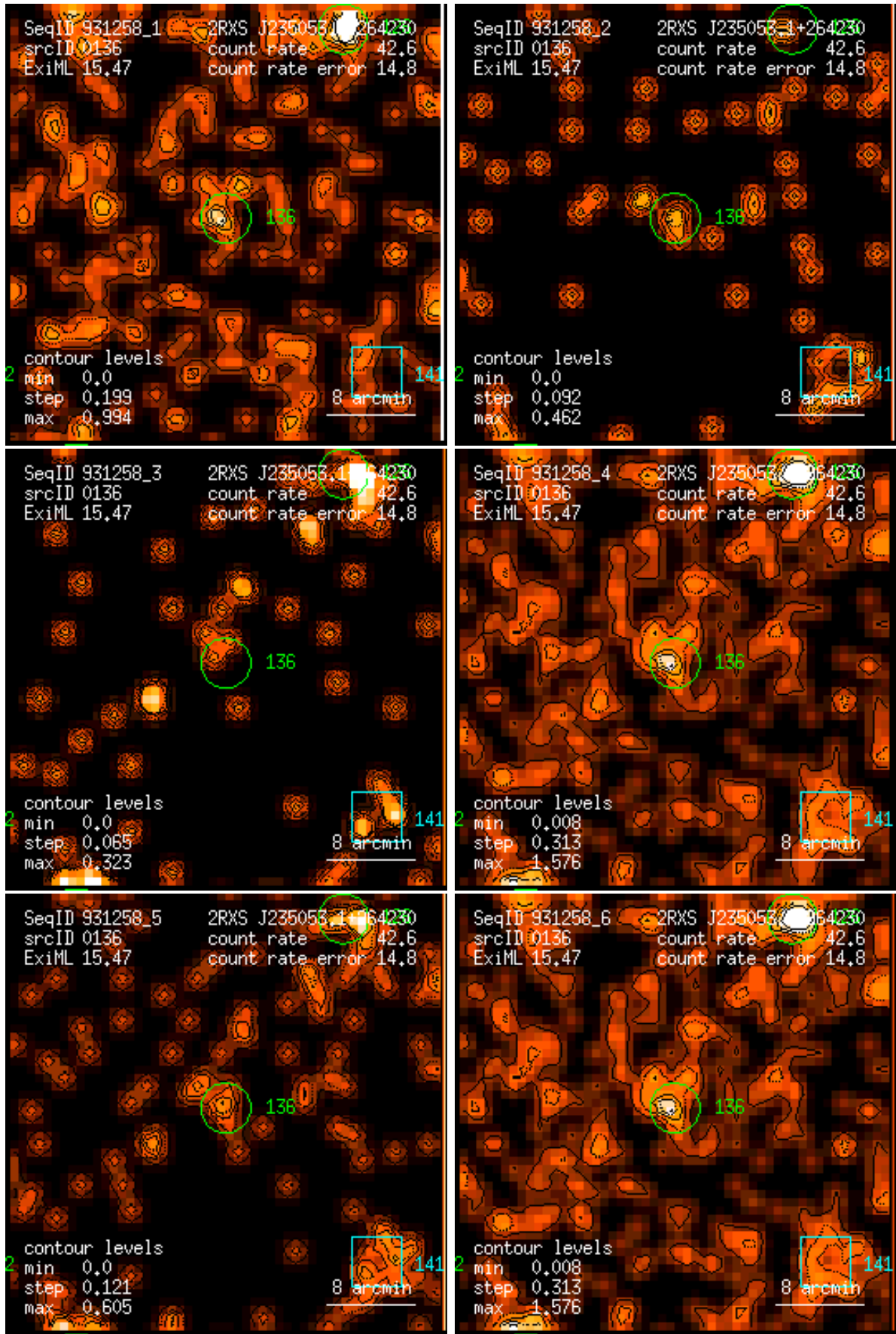
Figure 136: RASS 931258: detection 0136: band rate images, Gaussian filter: (1) PSPC channels 11 – 41, (2) 52 – 90, (3) 91 – 201, (4) 11 – 235, (5) 52 – 201, (6) 11 – 201. Broad band rates in counts/ks. Band rate contour levels in counts/ks/arcmin 2 .
