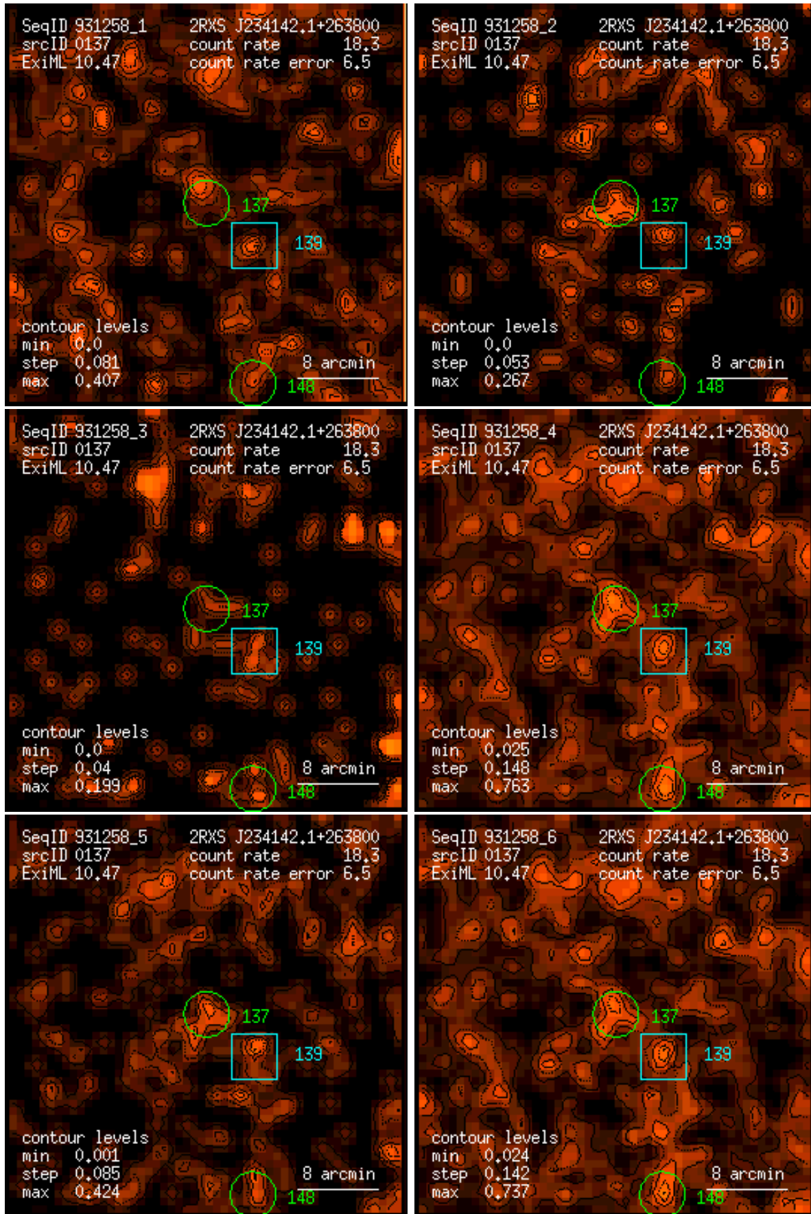
Figure 137: RASS 931258: detection 0137: band rate images, Gaussian filter: (1) PSPC channels 11 – 41, (2) 52 – 90, (3) 91 – 201, (4) 11 – 235, (5) 52 – 201, (6) 11 – 201. Broad band rates in counts/ks. Band rate contour levels in counts/ks/arcmin 2 .
