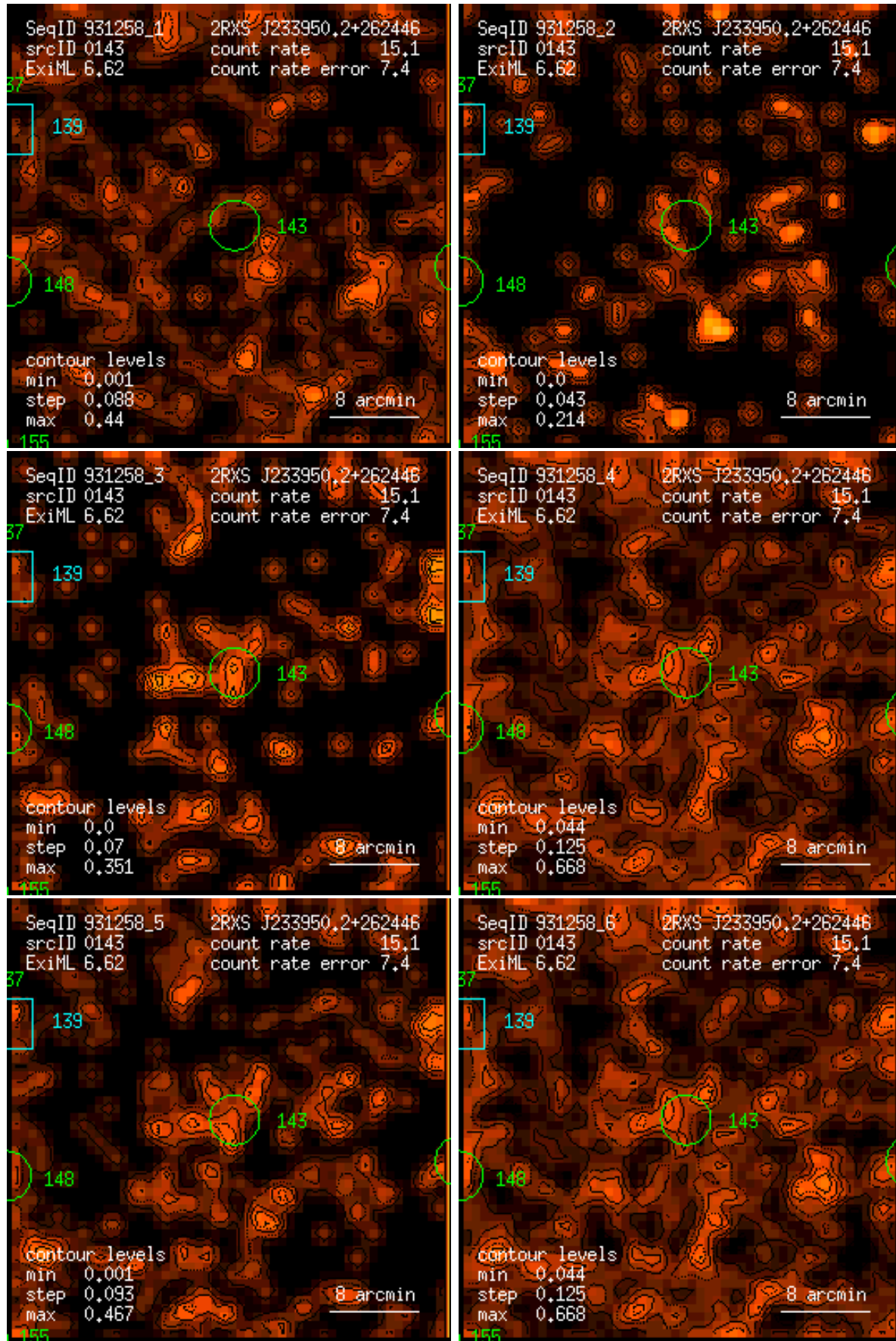
Figure 143: RASS 931258: detection 0143: band rate images, Gaussian filter: (1) PSPC channels 11 – 41, (2) 52 – 90, (3) 91 – 201, (4) 11 – 235, (5) 52 – 201, (6) 11 – 201. Broad band rates in counts/ks. Band rate contour levels in counts/ks/arcmin 2 .
