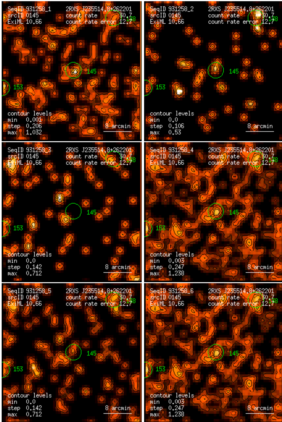
Figure 145: RASS 931258: detection 0145: band rate images, Gaussian filter: (1) PSPC channels 11 – 41, (2) 52 – 90, (3) 91 – 201, (4) 11 – 235, (5) 52 – 201, (6) 11 – 201. Broad band rates in counts/ks. Band rate contour levels in counts/ks/arcmin 2 .
