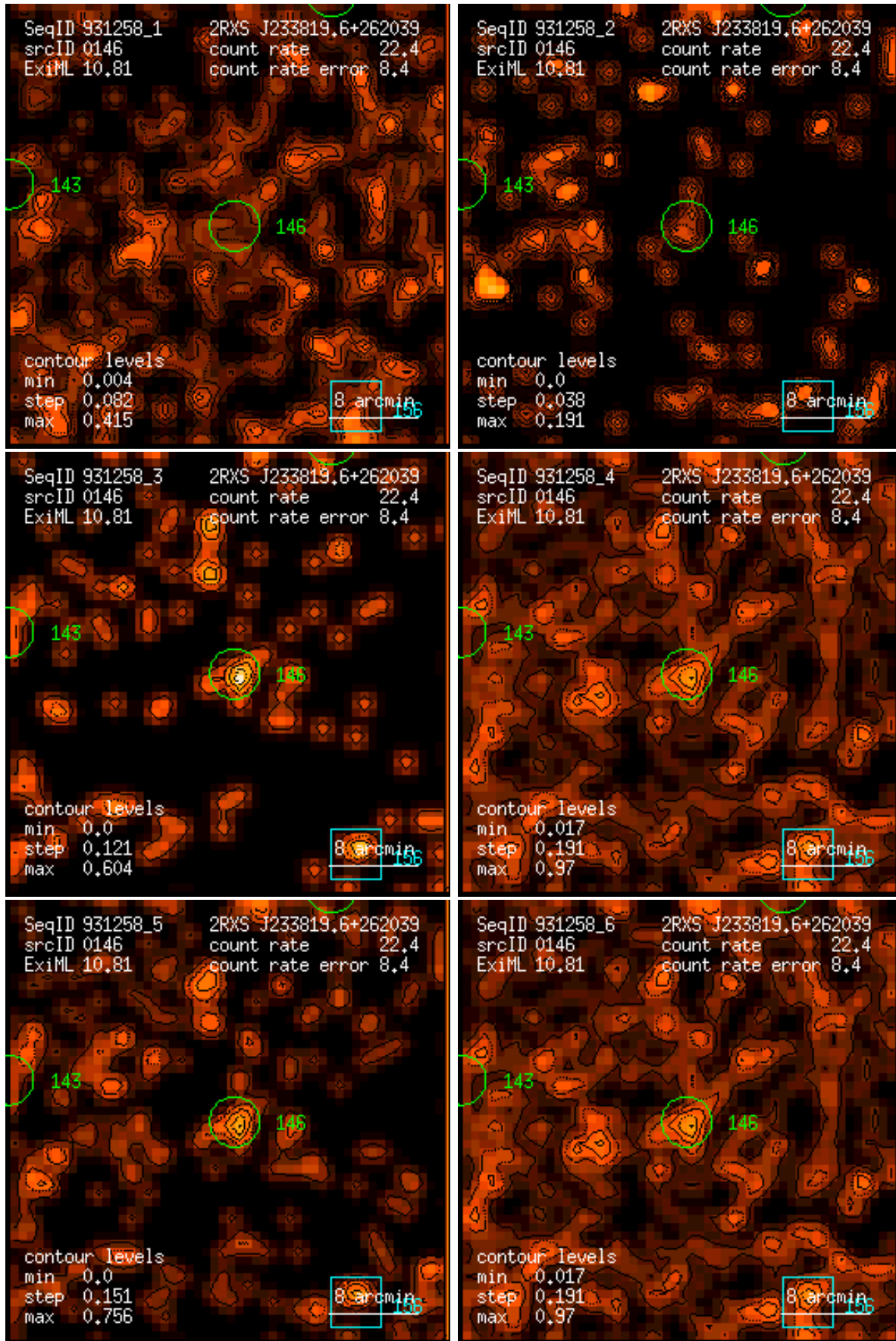
Figure 146: RASS 931258: detection 0146: band rate images, Gaussian filter: (1) PSPC channels 11 – 41, (2) 52 – 90, (3) 91 – 201, (4) 11 – 235, (5) 52 – 201, (6) 11 – 201. Broad band rates in counts/ks. Band rate contour levels in counts/ks/arcmin 2 .
