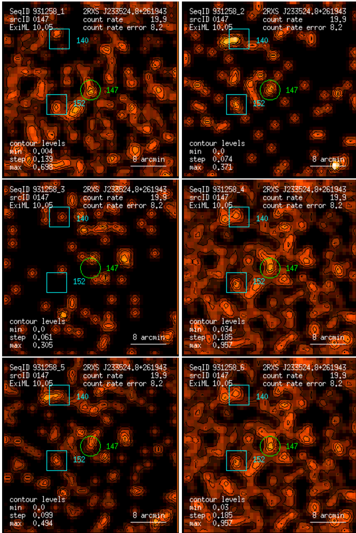
Figure 147: RASS 931258: detection 0147: band rate images, Gaussian filter: (1) PSPC channels 11 – 41, (2) 52 – 90, (3) 91 – 201, (4) 11 – 235, (5) 52 – 201, (6) 11 – 201. Broad band rates in counts/ks. Band rate contour levels in counts/ks/arcmin 2 .
