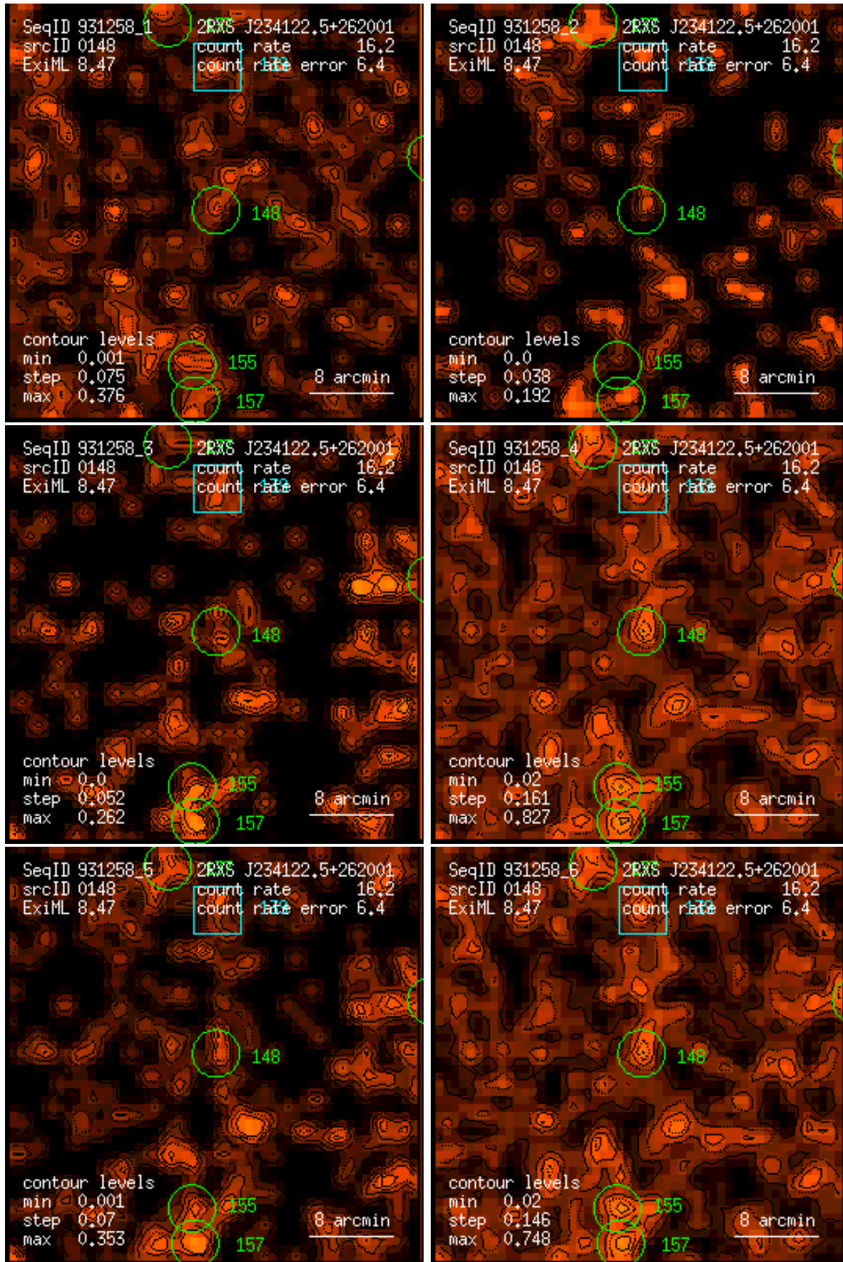
Figure 148: RASS 931258: detection 0148: band rate images, Gaussian filter: (1) PSPC channels 11 – 41, (2) 52 – 90, (3) 91 – 201, (4) 11 – 235, (5) 52 – 201, (6) 11 – 201. Broad band rates in counts/ks. Band rate contour levels in counts/ks/arcmin 2 .
