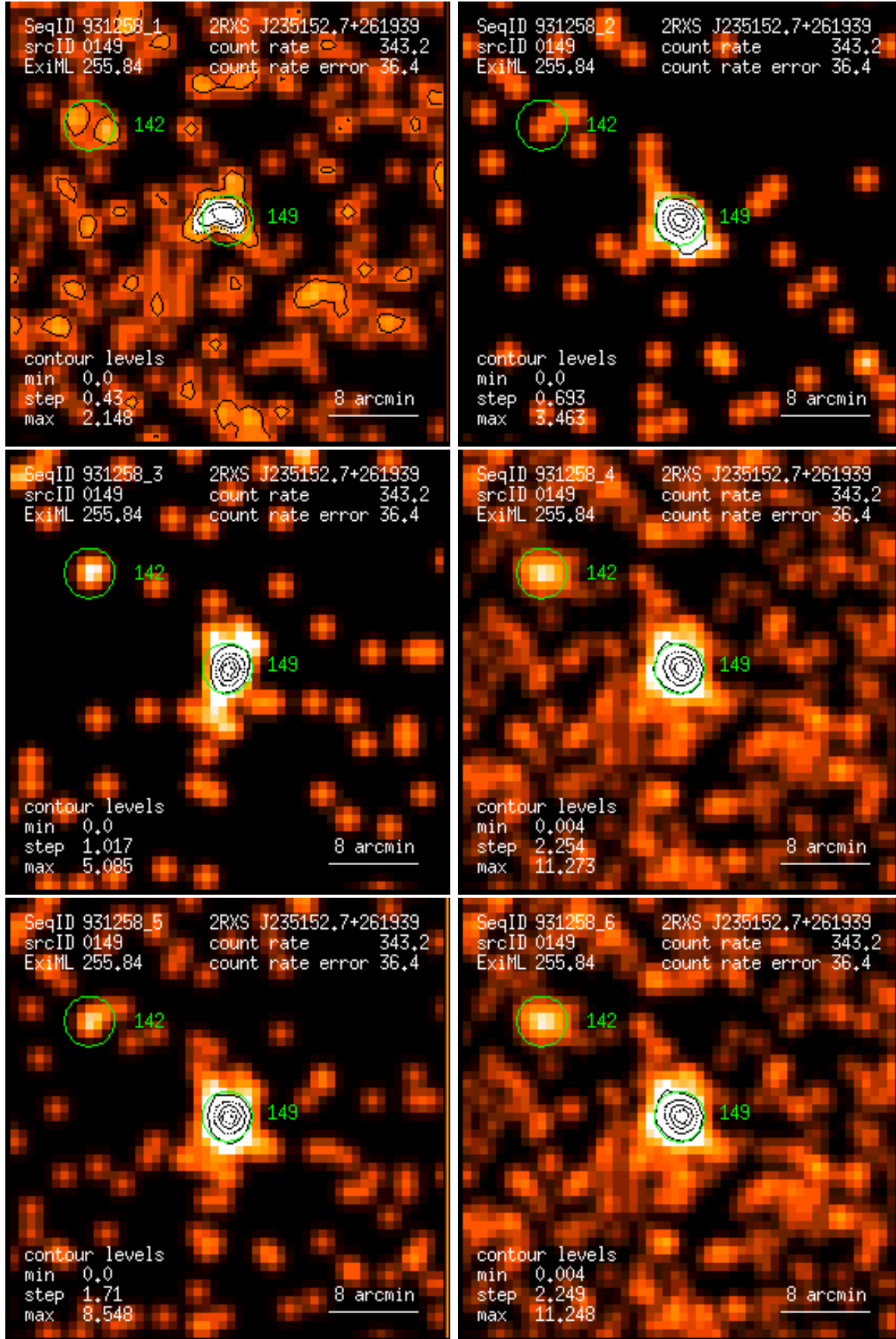
Figure 149: RASS 931258: detection 0149: band rate images, Gaussian filter: (1) PSPC channels 11 – 41, (2) 52 – 90, (3) 91 – 201, (4) 11 – 235, (5) 52 – 201, (6) 11 – 201. Broad band rates in counts/ks. Band rate contour levels in counts/ks/arcmin 2 .
