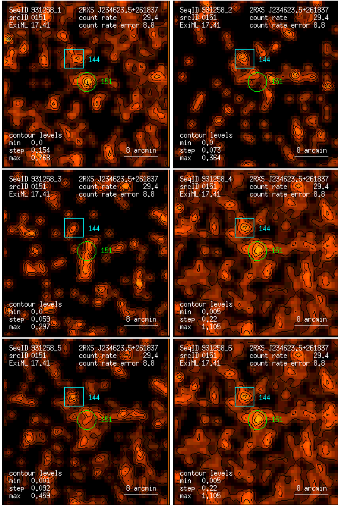
Figure 151: RASS 931258: detection 0151: band rate images, Gaussian filter: (1) PSPC channels 11 – 41, (2) 52 – 90, (3) 91 – 201, (4) 11 – 235, (5) 52 – 201, (6) 11 – 201. Broad band rates in counts/ks. Band rate contour levels in counts/ks/arcmin 2 .
