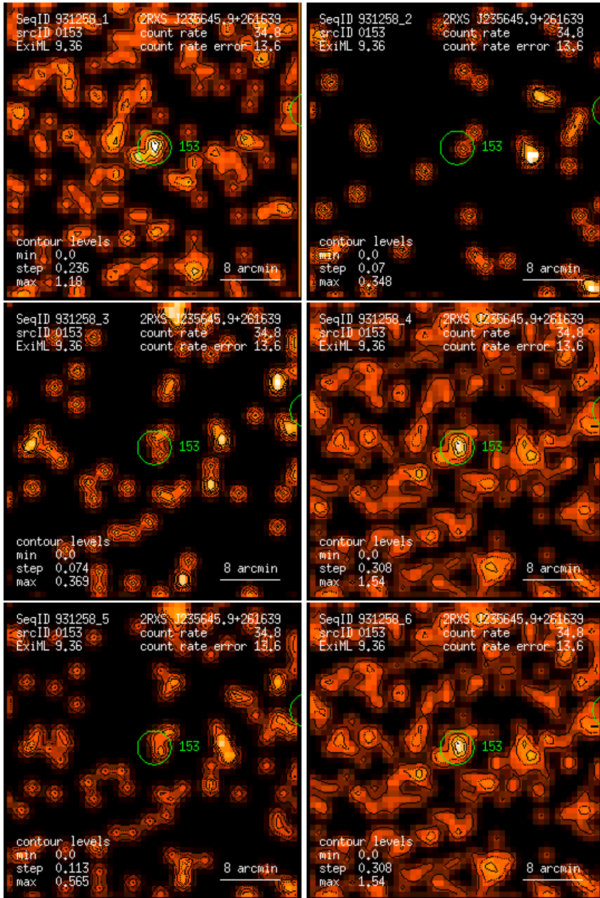
Figure 153: RASS 931258: detection 0153: band rate images, Gaussian filter: (1) PSPC channels 11 – 41, (2) 52 – 90, (3) 91 – 201, (4) 11 – 235, (5) 52 – 201, (6) 11 – 201. Broad band rates in counts/ks. Band rate contour levels in counts/ks/arcmin 2 .
