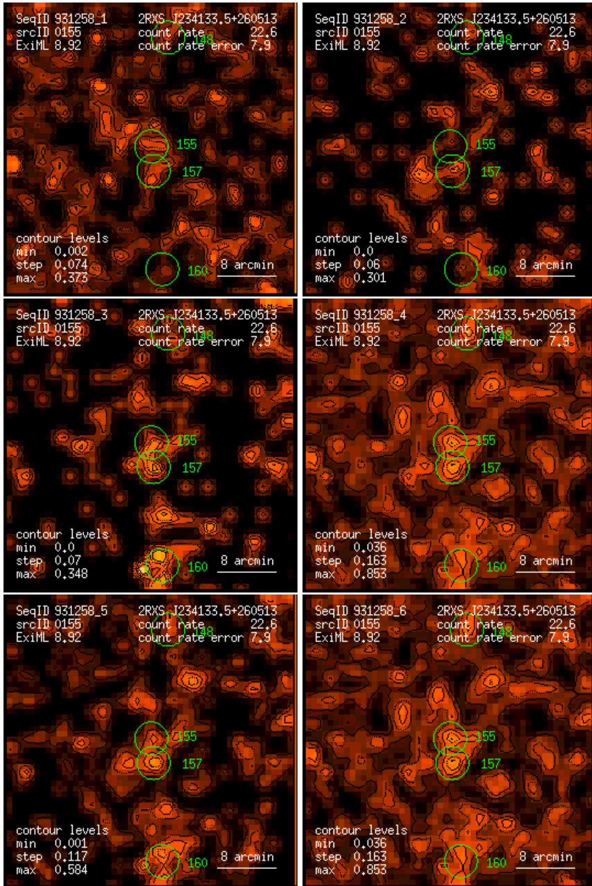
Figure 155: RASS 931258: detection 0155: band rate images, Gaussian filter: (1) PSPC channels 11 – 41, (2) 52 – 90, (3) 91 – 201, (4) 11 – 235, (5) 52 – 201, (6) 11 – 201. Broad band rates in counts/ks. Band rate contour levels in counts/ks/arcmin 2 .
