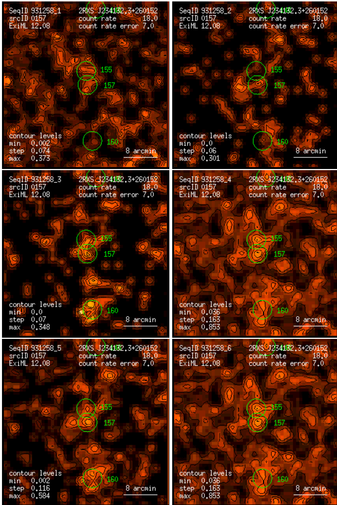
Figure 157: RASS 931258: detection 0157: band rate images, Gaussian filter: (1) PSPC channels 11 – 41, (2) 52 – 90, (3) 91 – 201, (4) 11 – 235, (5) 52 – 201, (6) 11 – 201. Broad band rates in counts/ks. Band rate contour levels in counts/ks/arcmin 2 .
