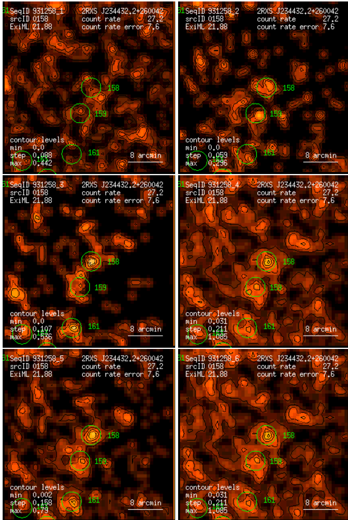
Figure 158: RASS 931258: detection 0158: band rate images, Gaussian filter: (1) PSPC channels 11 – 41, (2) 52 – 90, (3) 91 – 201, (4) 11 – 235, (5) 52 – 201, (6) 11 – 201. Broad band rates in counts/ks. Band rate contour levels in counts/ks/arcmin 2 .
