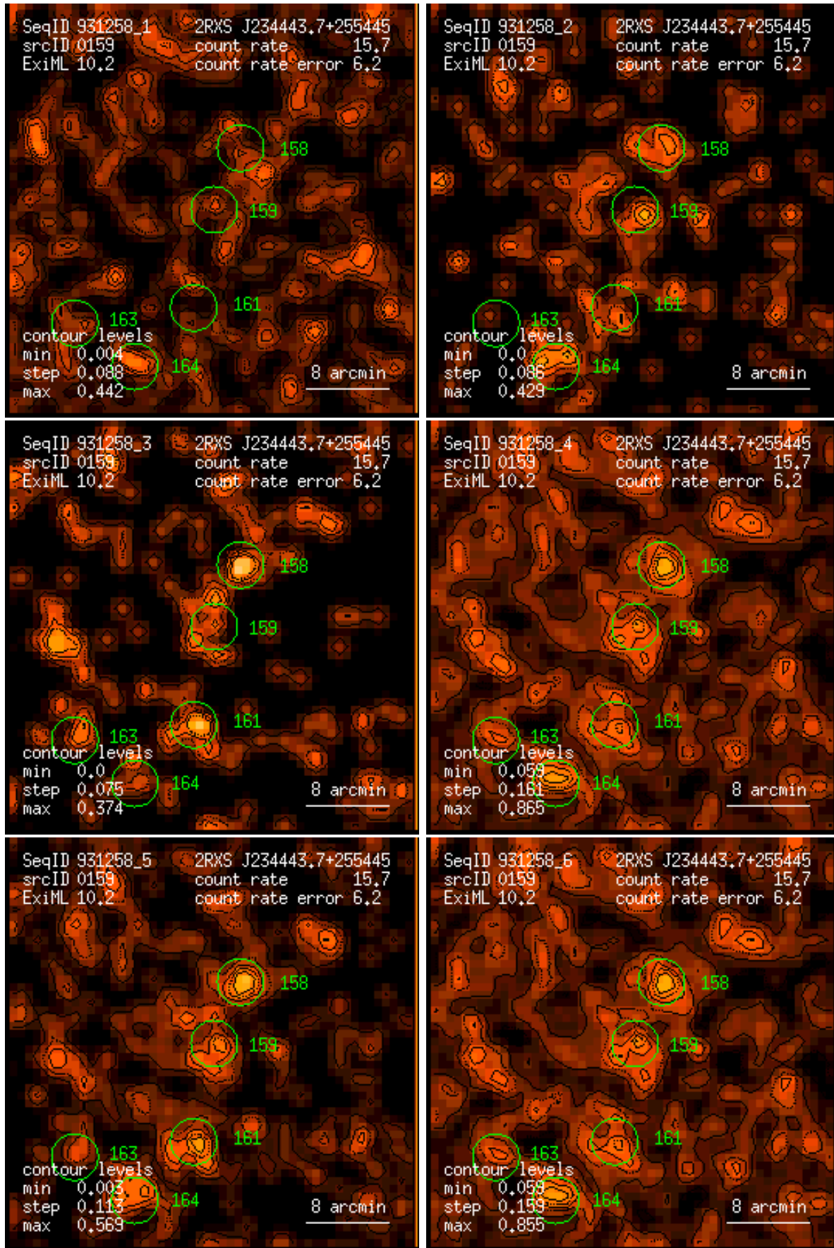
Figure 159: RASS 931258: detection 0159: band rate images, Gaussian filter: (1) PSPC channels 11 – 41, (2) 52 – 90, (3) 91 – 201, (4) 11 – 235, (5) 52 – 201, (6) 11 – 201. Broad band rates in counts/ks. Band rate contour levels in counts/ks/arcmin 2 .
