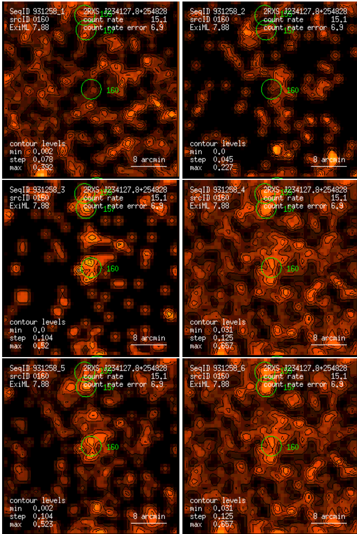
Figure 160: RASS 931258: detection 0160: band rate images, Gaussian filter: (1) PSPC channels 11 – 41, (2) 52 – 90, (3) 91 – 201, (4) 11 – 235, (5) 52 – 201, (6) 11 – 201. Broad band rates in counts/ks. Band rate contour levels in counts/ks/arcmin 2 .
