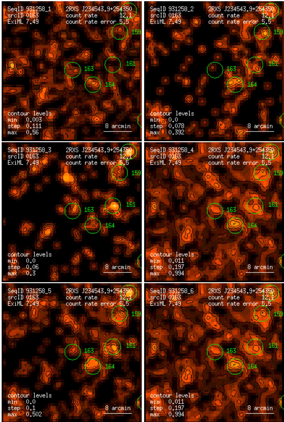
Figure 163: RASS 931258: detection 0163: band rate images, Gaussian filter: (1) PSPC channels 11 – 41, (2) 52 – 90, (3) 91 – 201, (4) 11 – 235, (5) 52 – 201, (6) 11 – 201. Broad band rates in counts/ks. Band rate contour levels in counts/ks/arcmin 2 .
