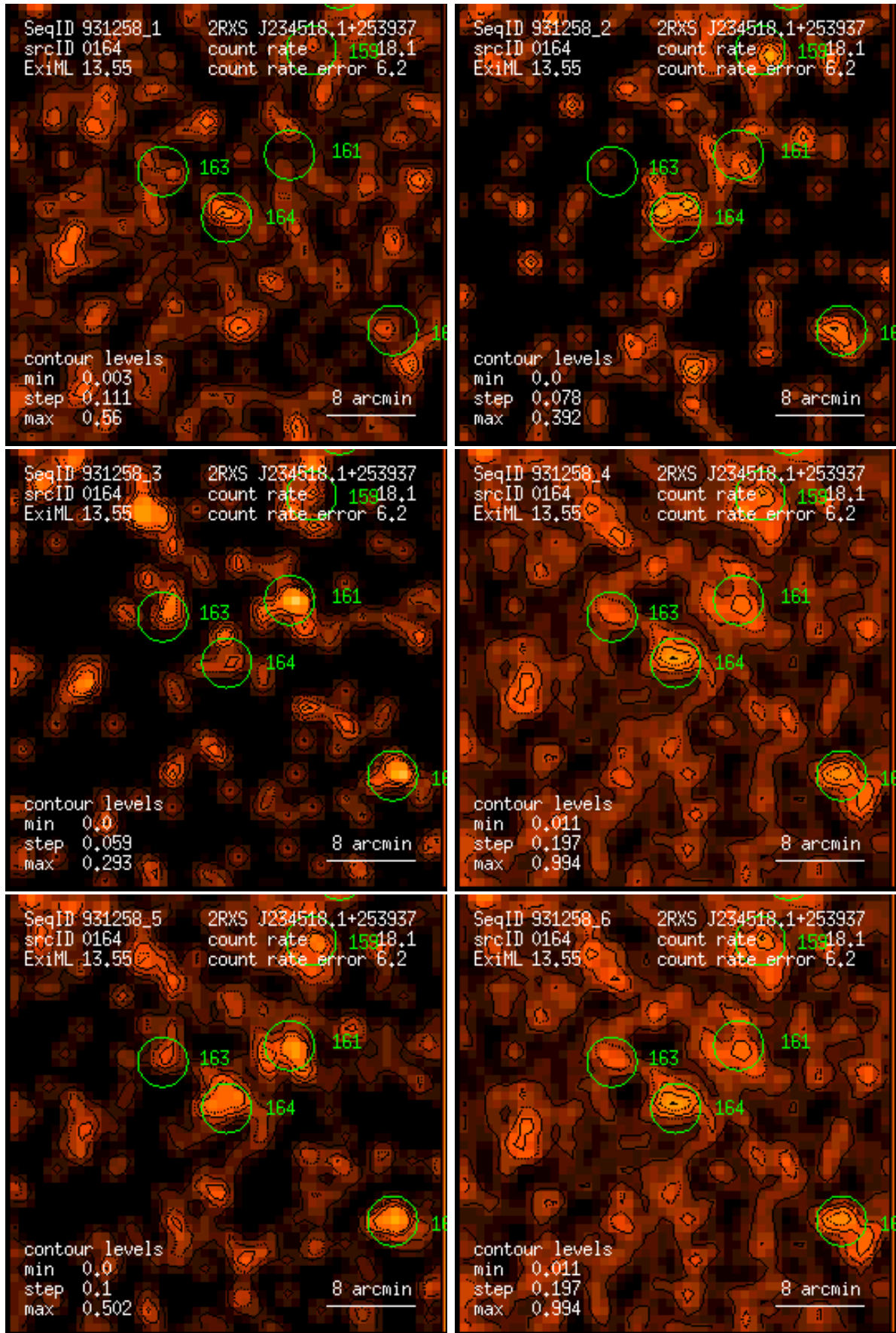
Figure 164: RASS 931258: detection 0164: band rate images, Gaussian filter: (1) PSPC channels 11 – 41, (2) 52 – 90, (3) 91 – 201, (4) 11 – 235, (5) 52 – 201, (6) 11 – 201. Broad band rates in counts/ks. Band rate contour levels in counts/ks/arcmin 2 .
