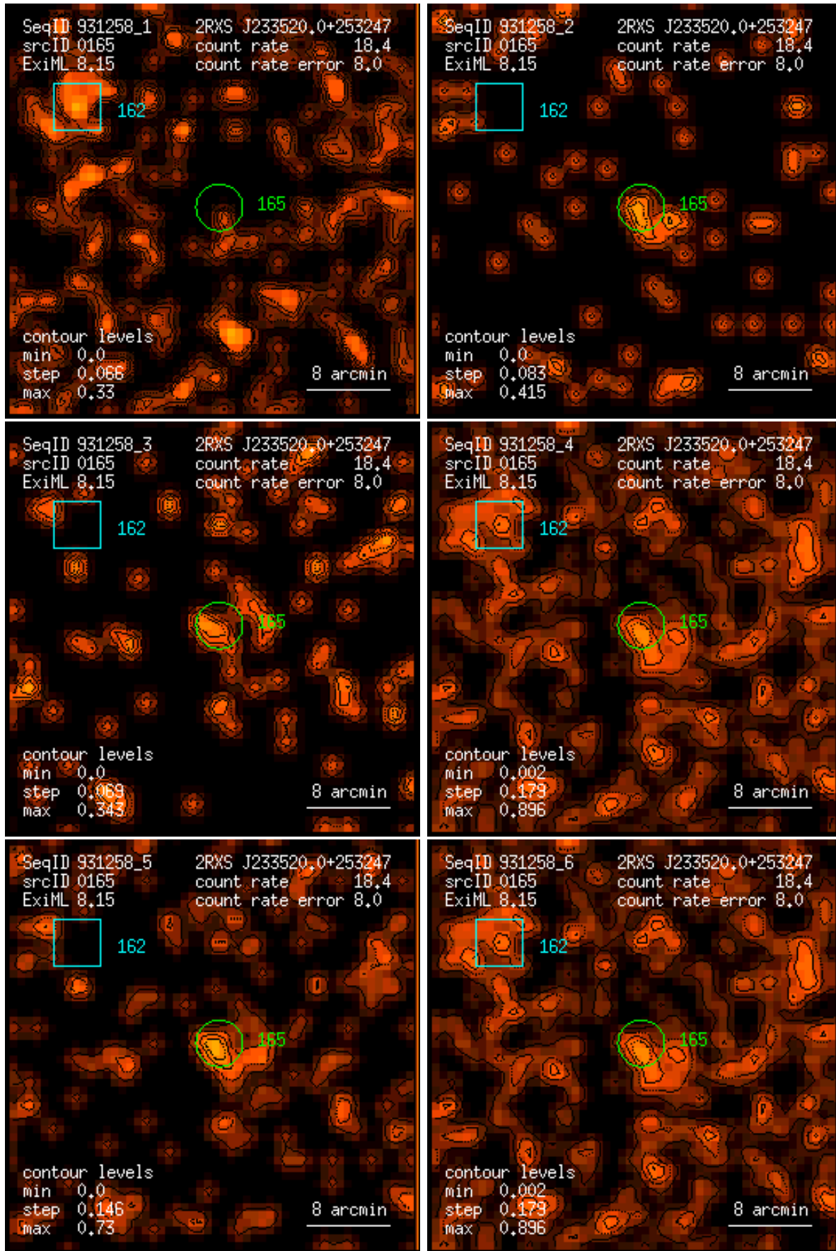
Figure 165: RASS 931258: detection 0165: band rate images, Gaussian filter: (1) PSPC channels 11 – 41, (2) 52 – 90, (3) 91 – 201, (4) 11 – 235, (5) 52 – 201, (6) 11 – 201. Broad band rates in counts/ks. Band rate contour levels in counts/ks/arcmin 2 .
