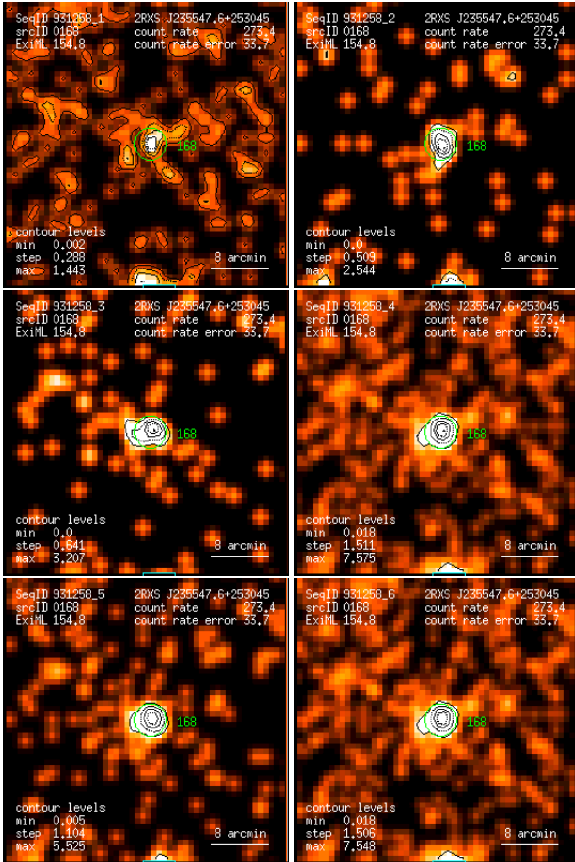
Figure 168: RASS 931258: detection 0168: band rate images, Gaussian filter: (1) PSPC channels 11 – 41, (2) 52 – 90, (3) 91 – 201, (4) 11 – 235, (5) 52 – 201, (6) 11 – 201. Broad band rates in counts/ks. Band rate contour levels in counts/ks/arcmin 2 .
