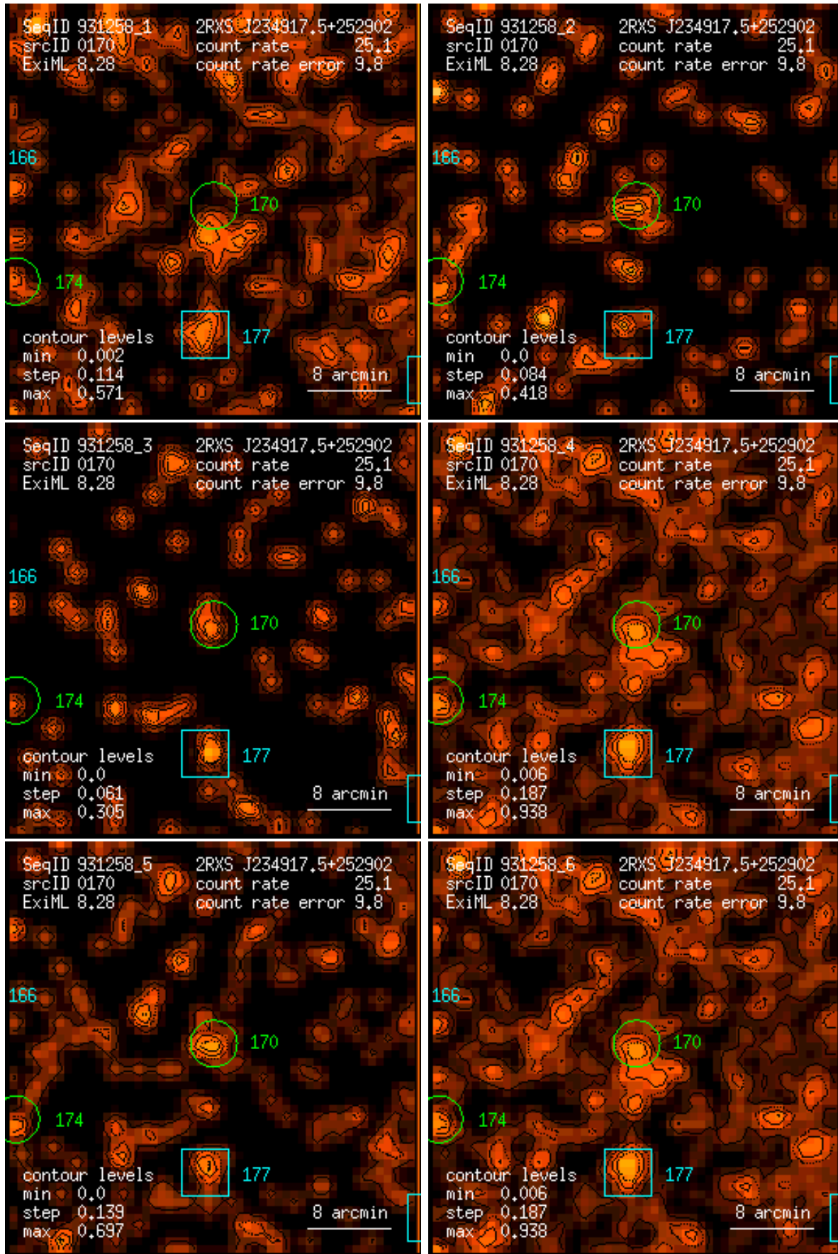
Figure 170: RASS 931258: detection 0170: band rate images, Gaussian filter: (1) PSPC channels 11 – 41, (2) 52 – 90, (3) 91 – 201, (4) 11 – 235, (5) 52 – 201, (6) 11 – 201. Broad band rates in counts/ks. Band rate contour levels in counts/ks/arcmin 2 .
