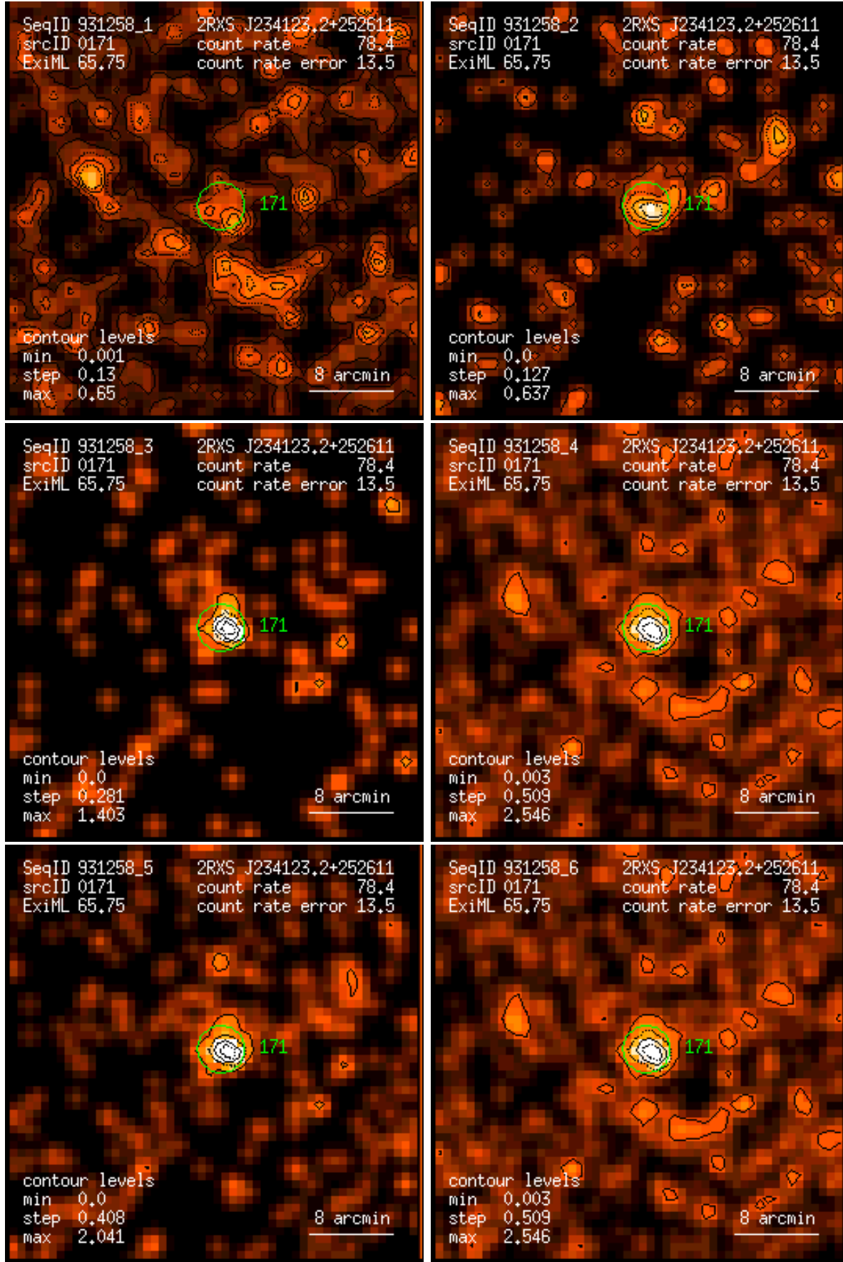
Figure 171: RASS 931258: detection 0171: band rate images, Gaussian filter: (1) PSPC channels 11 – 41, (2) 52 – 90, (3) 91 – 201, (4) 11 – 235, (5) 52 – 201, (6) 11 – 201. Broad band rates in counts/ks. Band rate contour levels in counts/ks/arcmin 2 .
