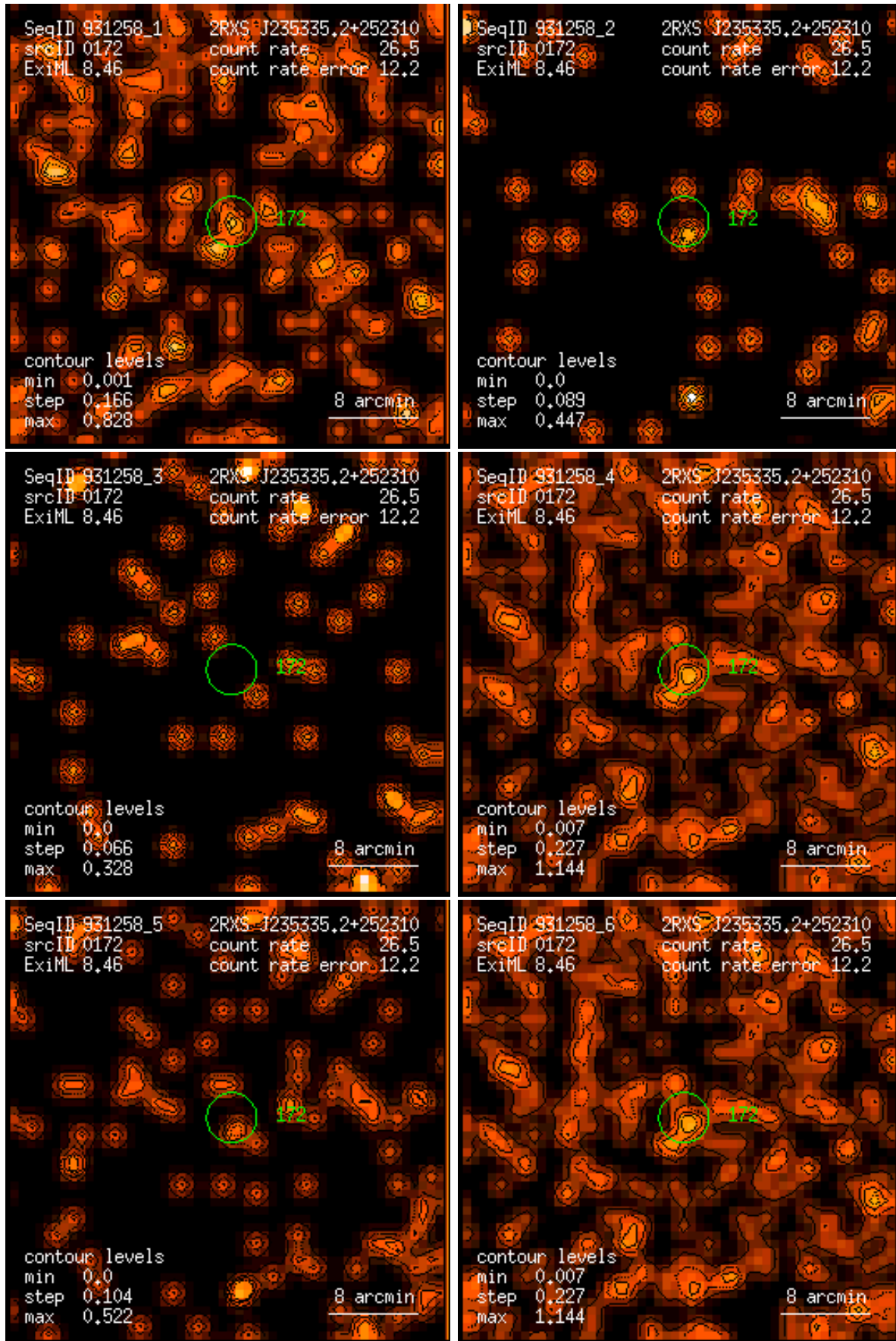
Figure 172: RASS 931258: detection 0172: band rate images, Gaussian filter: (1) PSPC channels 11 – 41, (2) 52 – 90, (3) 91 – 201, (4) 11 – 235, (5) 52 – 201, (6) 11 – 201. Broad band rates in counts/ks. Band rate contour levels in counts/ks/arcmin 2 .
