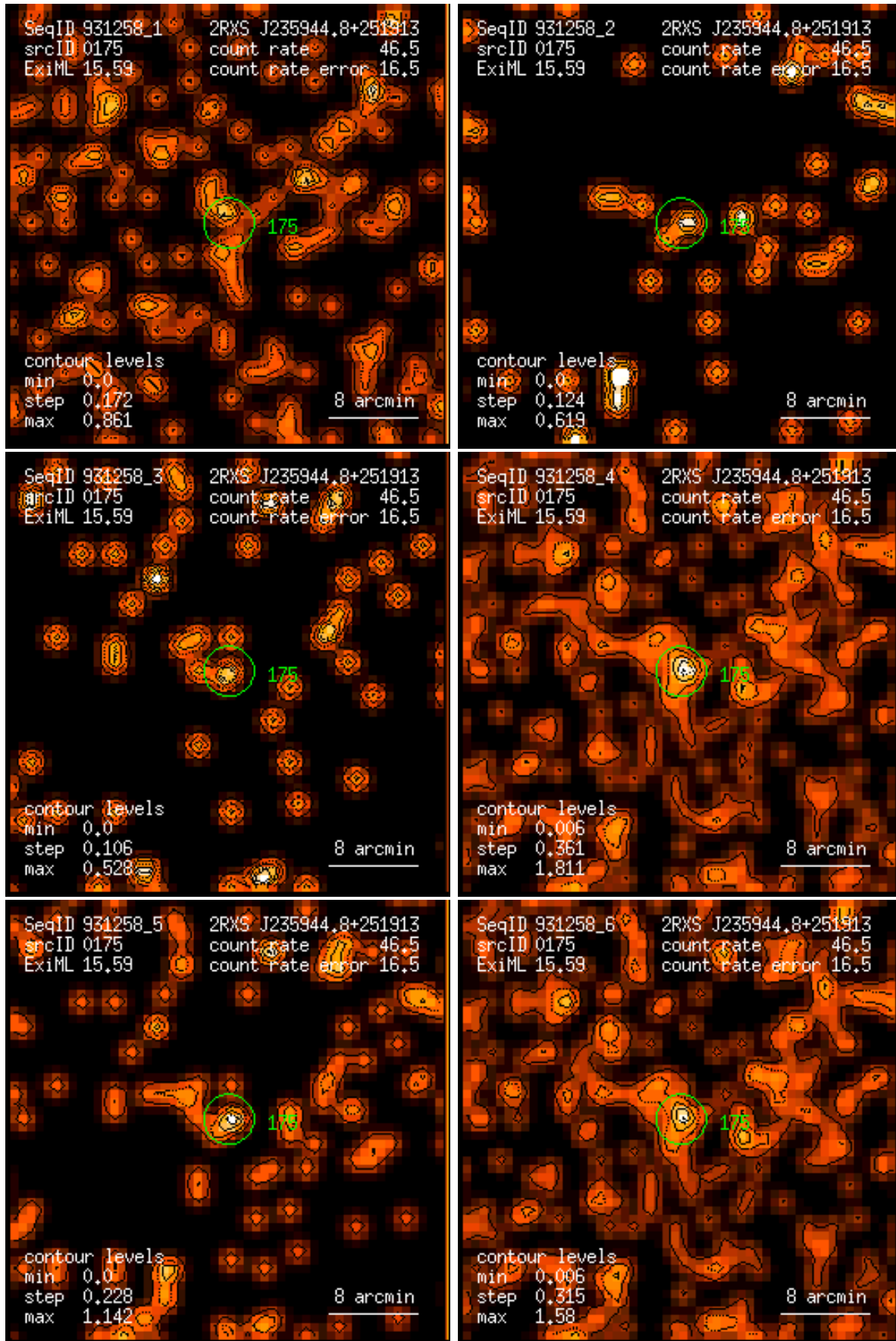
Figure 175: RASS 931258: detection 0175: band rate images, Gaussian filter: (1) PSPC channels 11 – 41, (2) 52 – 90, (3) 91 – 201, (4) 11 – 235, (5) 52 – 201, (6) 11 – 201. Broad band rates in counts/ks. Band rate contour levels in counts/ks/arcmin 2 .
