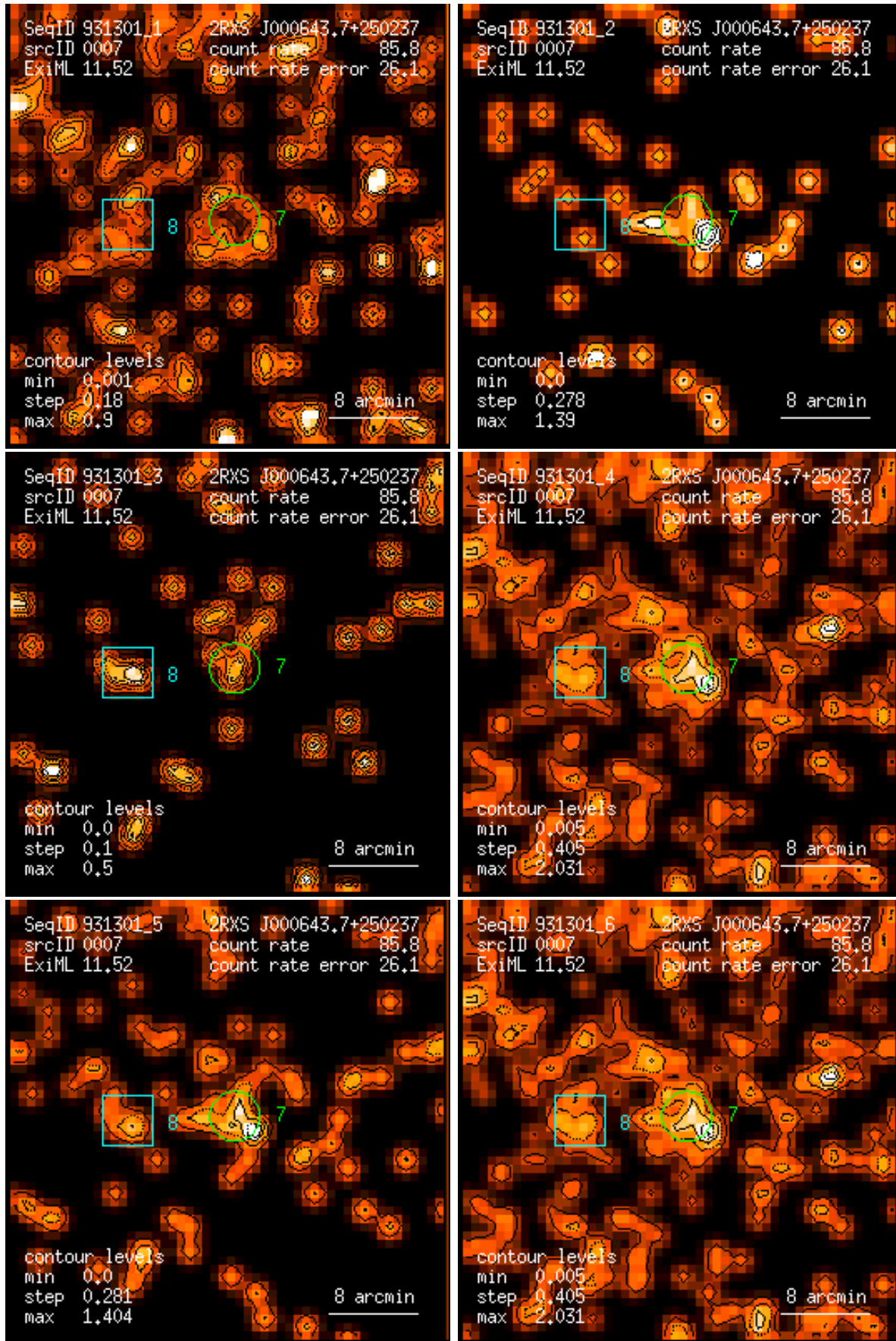
Figure 7: RASS 931301: detection 0007: band rate images, Gaussian filter: (1) PSPC channels 11 – 41, (2) 52 – 90, (3) 91 – 201, (4) 11 – 235, (5) 52 – 201, (6) 11 – 201. Broad band rates in counts/ks. Band rate contour levels in counts/ks/arcmin 2 .
