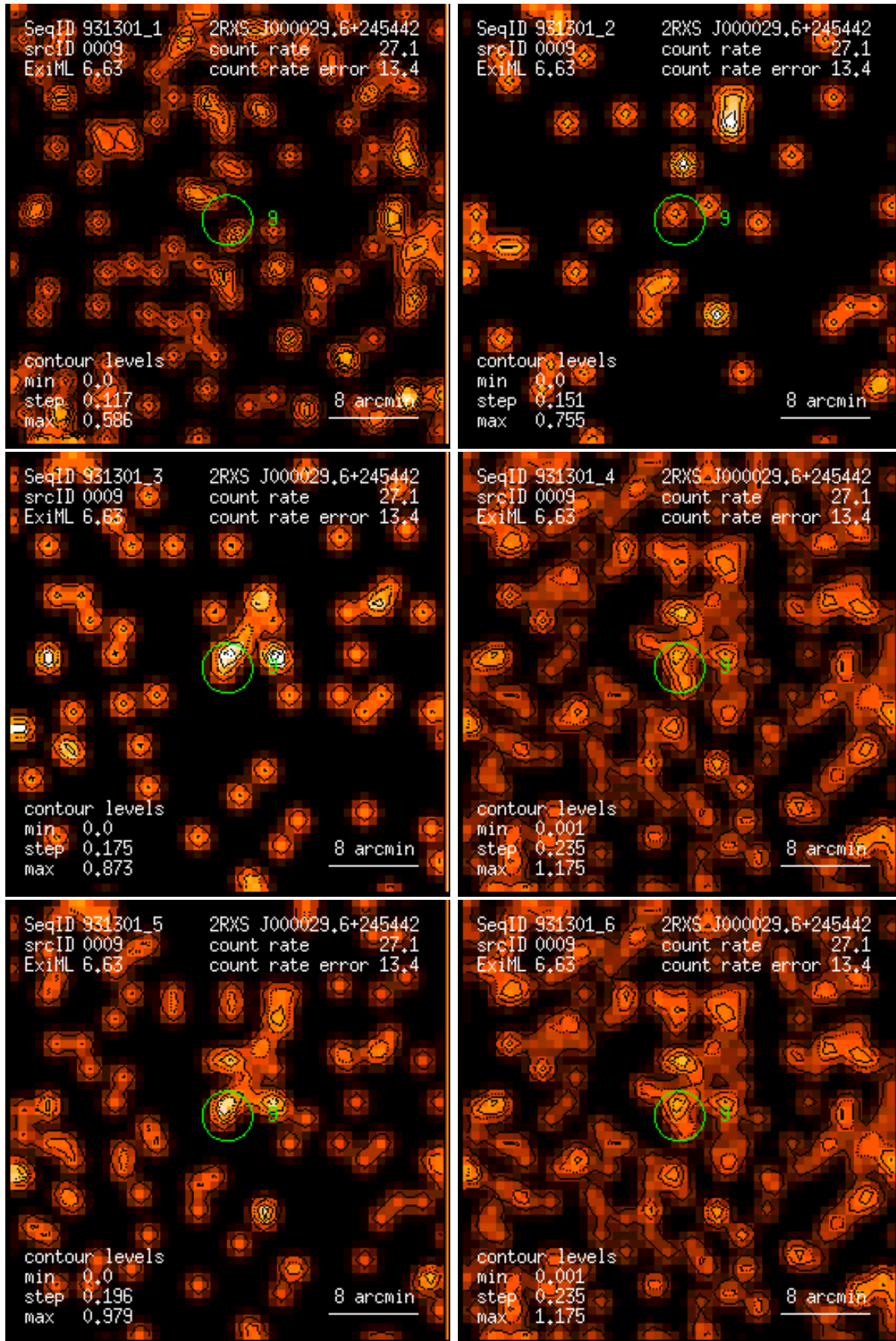
Figure 9: RASS 931301: detection 0009: band rate images, Gaussian filter: (1) PSPC channels 11 – 41, (2) 52 – 90, (3) 91 – 201, (4) 11 – 235, (5) 52 – 201, (6) 11 – 201. Broad band rates in counts/ks. Band rate contour levels in counts/ks/arcmin 2 .
