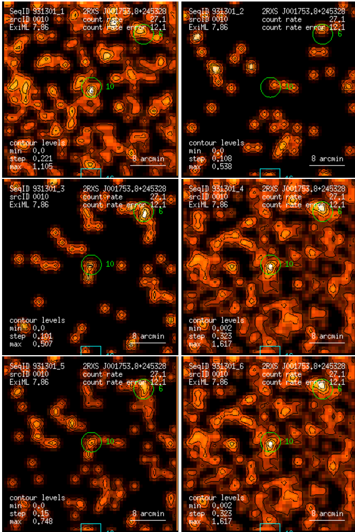
Figure 10: RASS 931301: detection 0010: band rate images, Gaussian filter: (1) PSPC channels 11 – 41, (2) 52 – 90, (3) 91 – 201, (4) 11 – 235, (5) 52 – 201, (6) 11 – 201. Broad band rates in counts/ks. Band rate contour levels in counts/ks/arcmin 2 .
