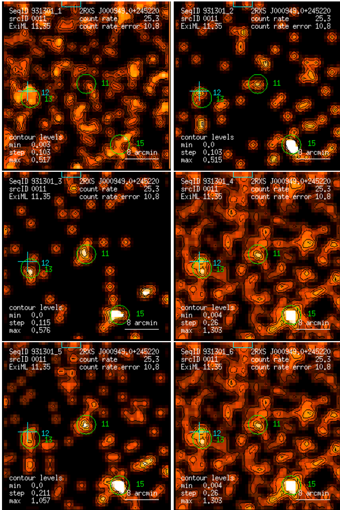
Figure 11: RASS 931301: detection 0011: band rate images, Gaussian filter: (1) PSPC channels 11 – 41, (2) 52 – 90, (3) 91 – 201, (4) 11 – 235, (5) 52 – 201, (6) 11 – 201. Broad band rates in counts/ks. Band rate contour levels in counts/ks/arcmin 2 .
