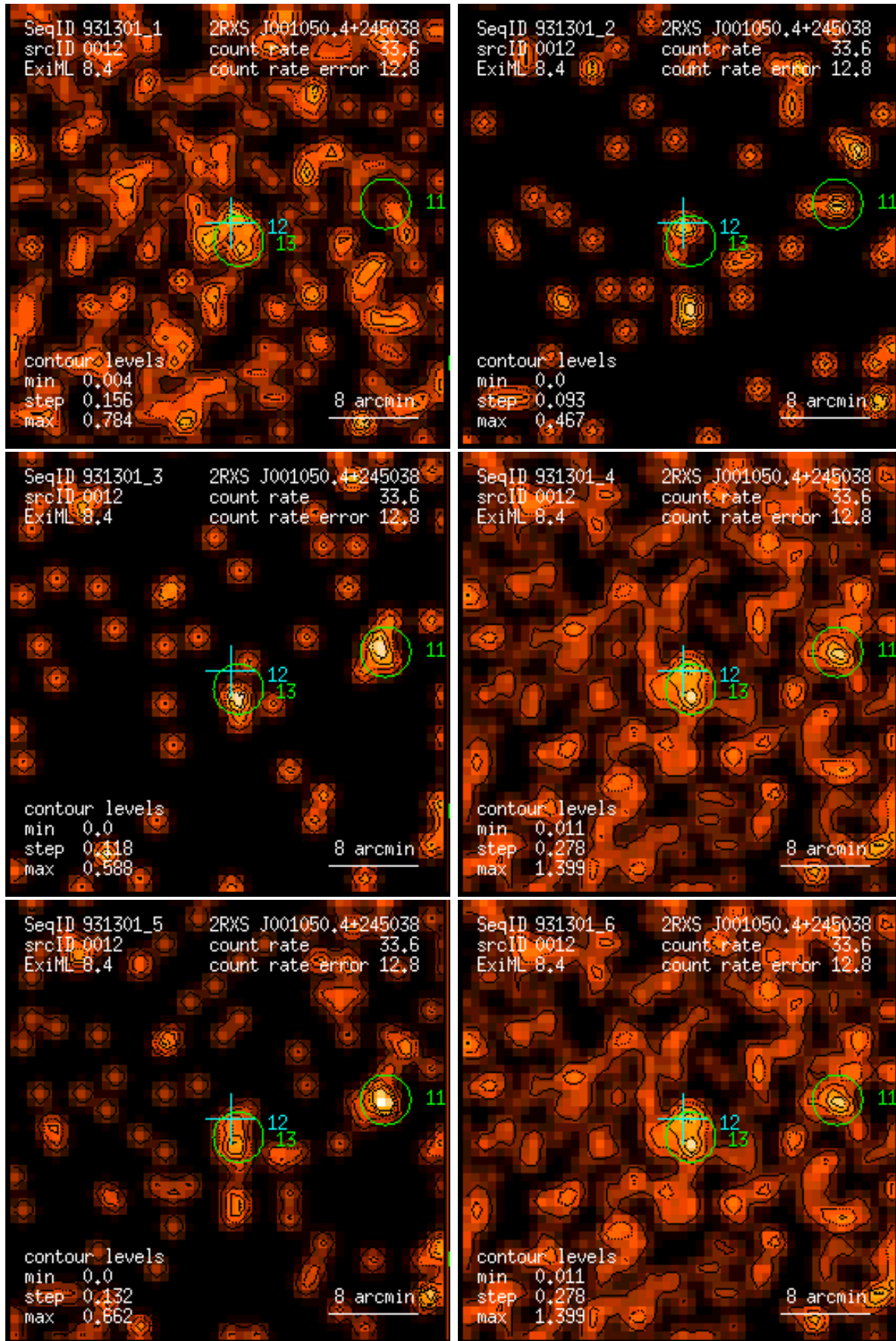
Figure 12: RASS 931301: detection 0012: band rate images, Gaussian filter: (1) PSPC channels 11 – 41, (2) 52 – 90, (3) 91 – 201, (4) 11 – 235, (5) 52 – 201, (6) 11 – 201. Broad band rates in counts/ks. Band rate contour levels in counts/ks/arcmin 2 .
