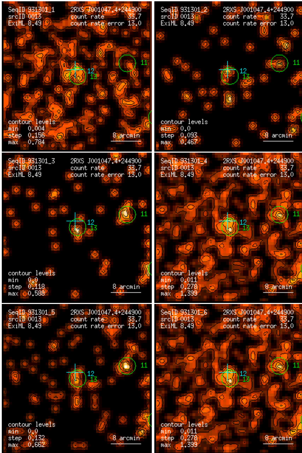
Figure 13: RASS 931301: detection 0013: band rate images, Gaussian filter: (1) PSPC channels 11 – 41, (2) 52 – 90, (3) 91 – 201, (4) 11 – 235, (5) 52 – 201, (6) 11 – 201. Broad band rates in counts/ks. Band rate contour levels in counts/ks/arcmin 2 .
