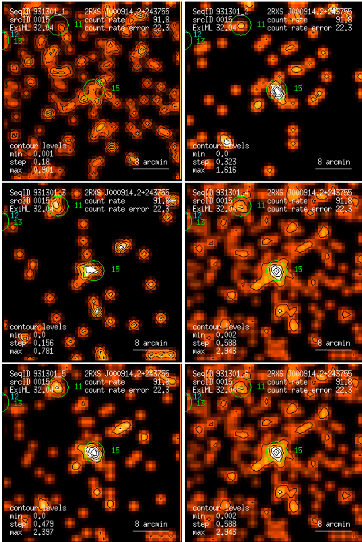
Figure 15: RASS 931301: detection 0015: band rate images, Gaussian filter: (1) PSPC channels 11 – 41, (2) 52 – 90, (3) 91 – 201, (4) 11 – 235, (5) 52 – 201, (6) 11 – 201. Broad band rates in counts/ks. Band rate contour levels in counts/ks/arcmin 2 .
