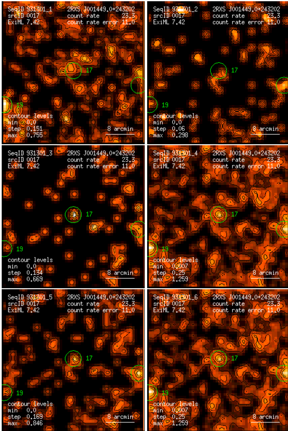
Figure 17: RASS 931301: detection 0017: band rate images, Gaussian filter: (1) PSPC channels 11 – 41, (2) 52 – 90, (3) 91 – 201, (4) 11 – 235, (5) 52 – 201, (6) 11 – 201. Broad band rates in counts/ks. Band rate contour levels in counts/ks/arcmin 2 .
