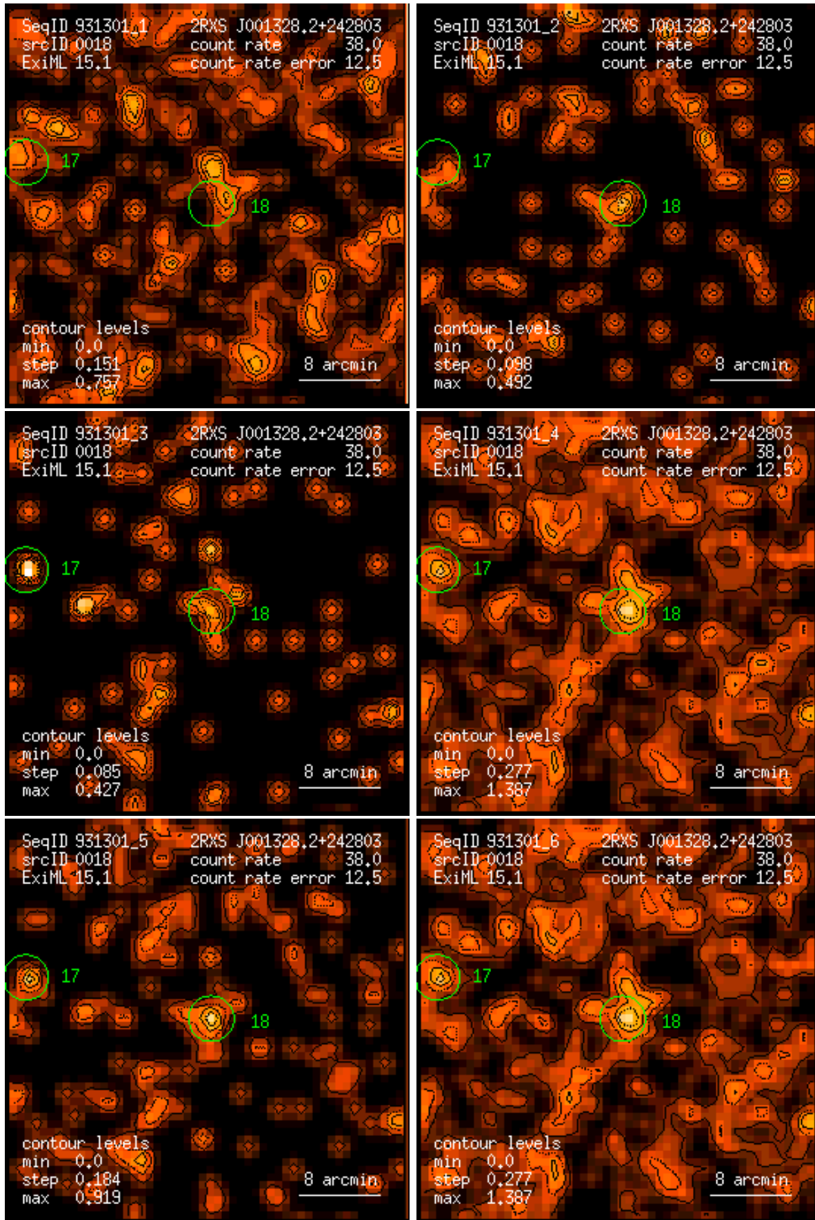
Figure 18: RASS 931301: detection 0018: band rate images, Gaussian filter: (1) PSPC channels 11 – 41, (2) 52 – 90, (3) 91 – 201, (4) 11 – 235, (5) 52 – 201, (6) 11 – 201. Broad band rates in counts/ks. Band rate contour levels in counts/ks/arcmin 2 .
