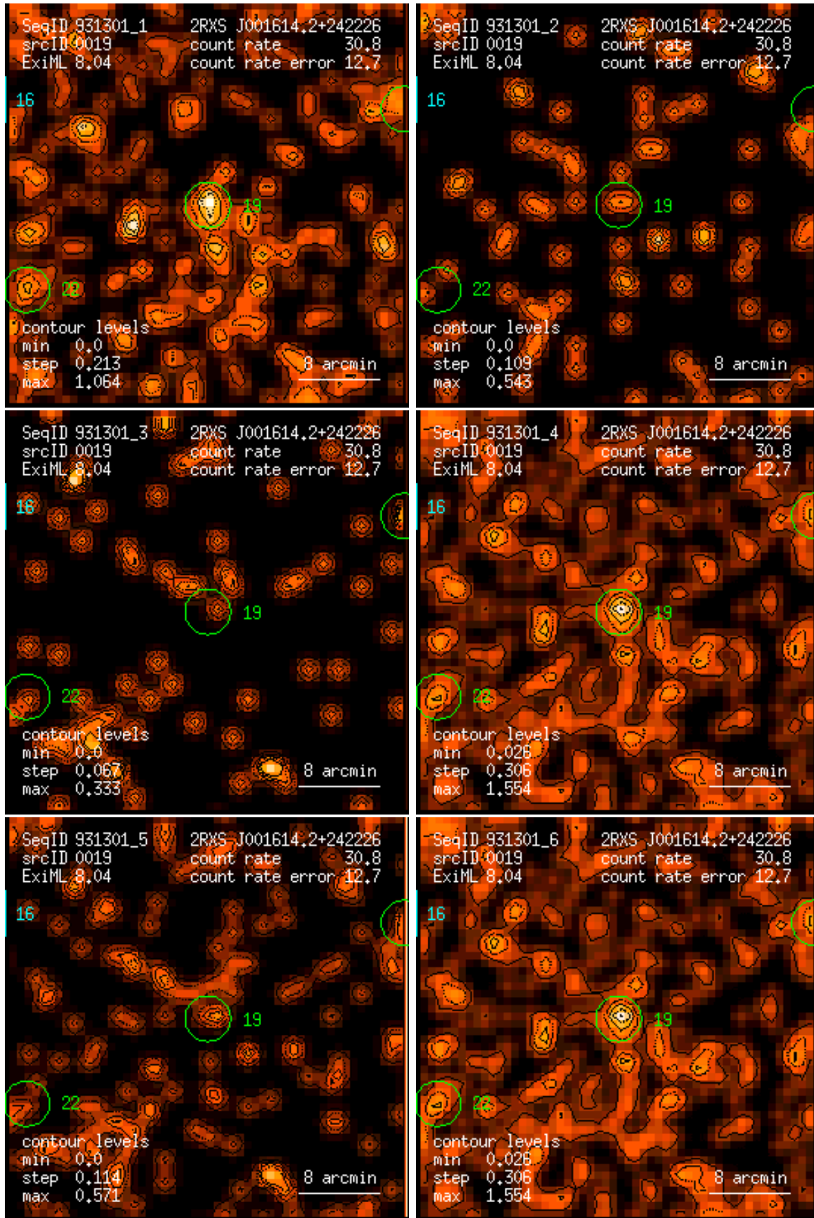
Figure 19: RASS 931301: detection 0019: band rate images, Gaussian filter: (1) PSPC channels 11 – 41, (2) 52 – 90, (3) 91 – 201, (4) 11 – 235, (5) 52 – 201, (6) 11 – 201. Broad band rates in counts/ks. Band rate contour levels in counts/ks/arcmin 2 .
