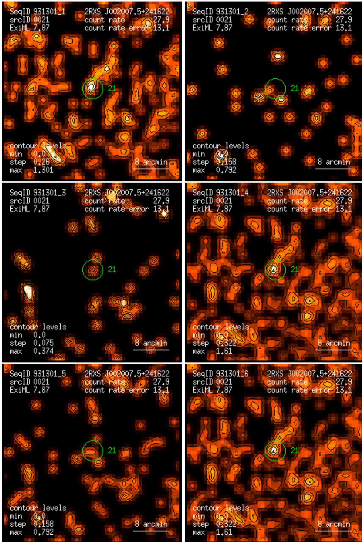
Figure 21: RASS 931301: detection 0021: band rate images, Gaussian filter: (1) PSPC channels 11 – 41, (2) 52 – 90, (3) 91 – 201, (4) 11 – 235, (5) 52 – 201, (6) 11 – 201. Broad band rates in counts/ks. Band rate contour levels in counts/ks/arcmin 2 .
