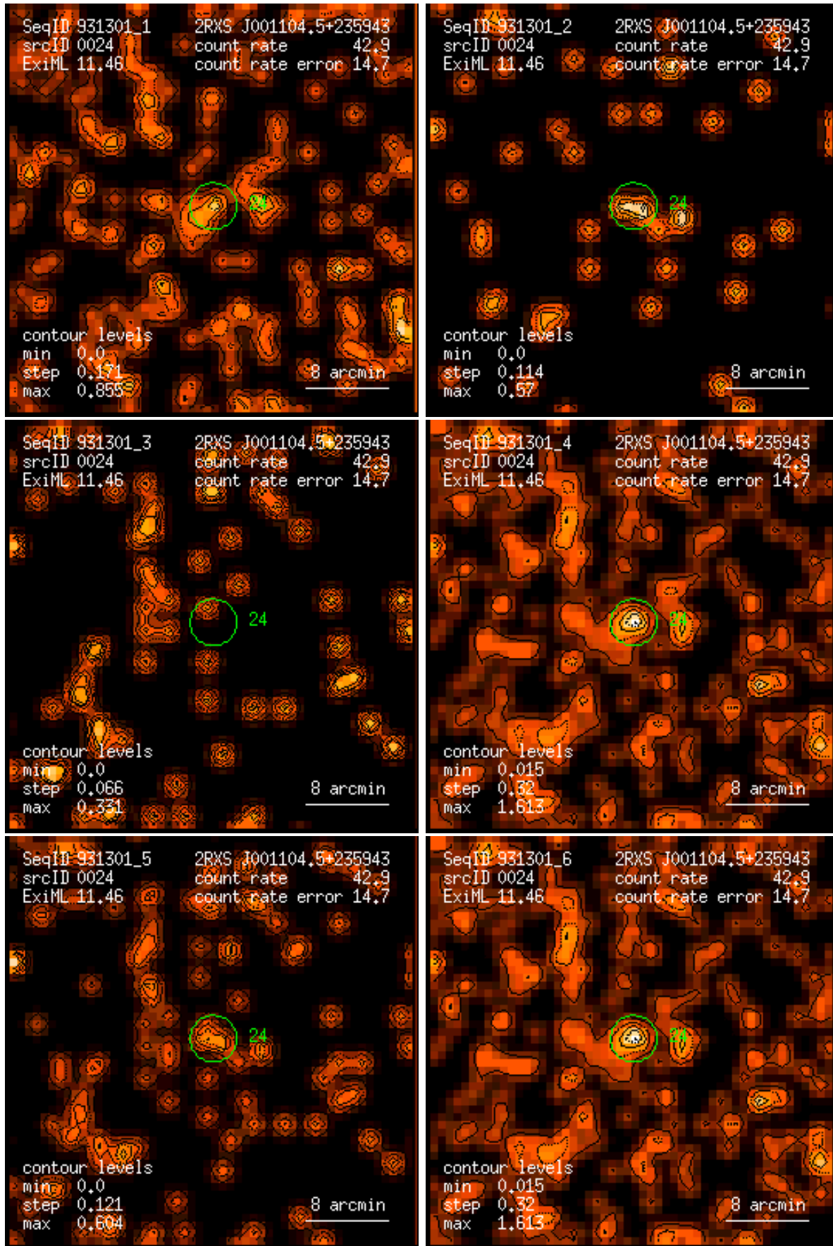
Figure 24: RASS 931301: detection 0024: band rate images, Gaussian filter: (1) PSPC channels 11 – 41, (2) 52 – 90, (3) 91 – 201, (4) 11 – 235, (5) 52 – 201, (6) 11 – 201. Broad band rates in counts/ks. Band rate contour levels in counts/ks/arcmin 2 .
