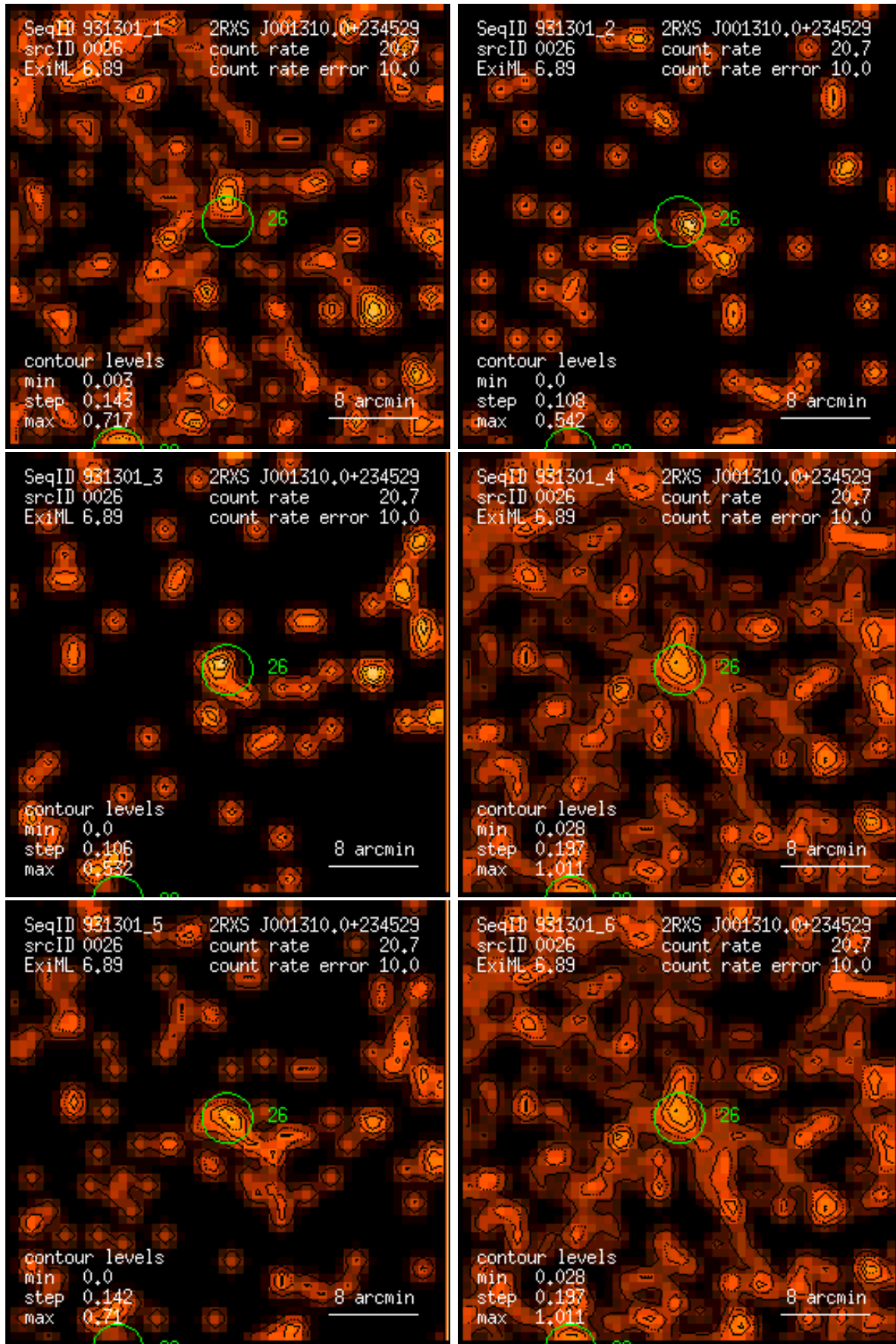
Figure 26: RASS 931301: detection 0026: band rate images, Gaussian filter: (1) PSPC channels 11 – 41, (2) 52 – 90, (3) 91 – 201, (4) 11 – 235, (5) 52 – 201, (6) 11 – 201. Broad band rates in counts/ks. Band rate contour levels in counts/ks/arcmin 2 .
