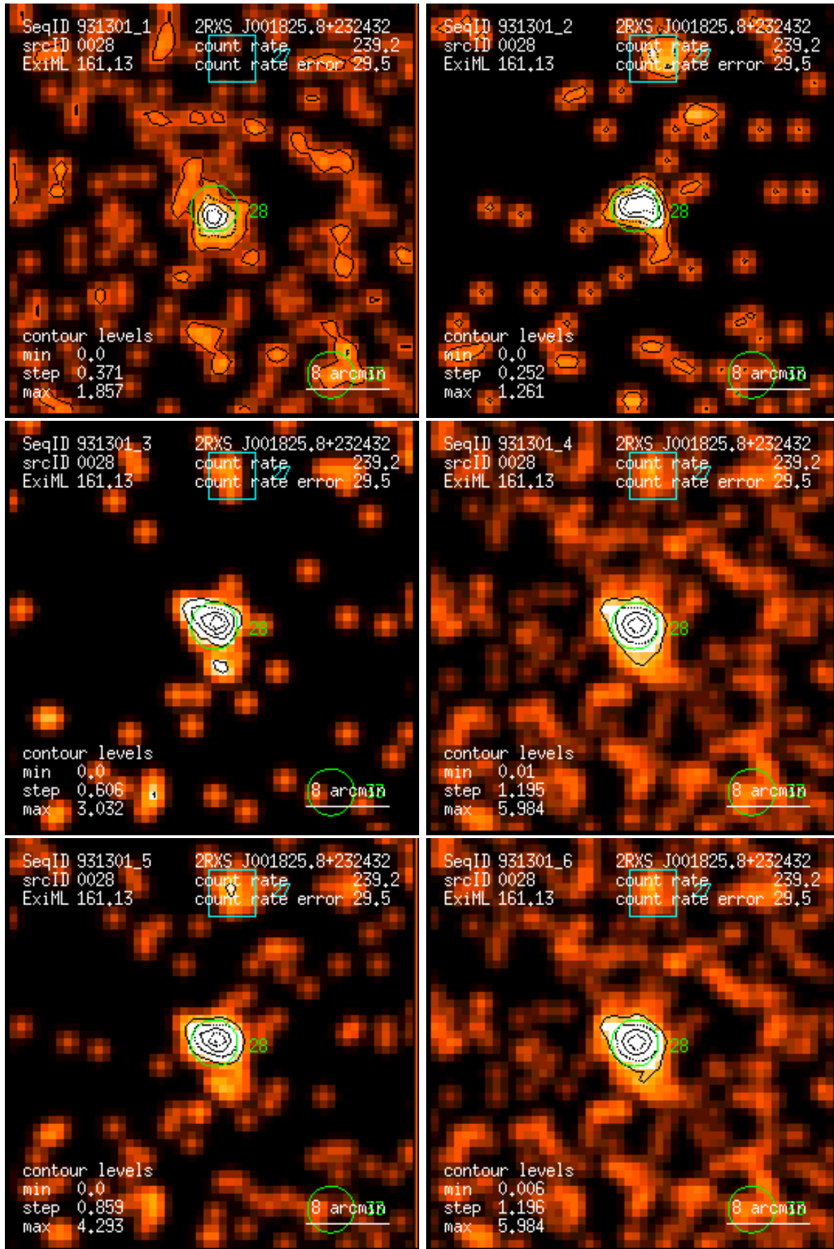
Figure 28: RASS 931301: detection 0028: band rate images, Gaussian filter: (1) PSPC channels 11 – 41, (2) 52 – 90, (3) 91 – 201, (4) 11 – 235, (5) 52 – 201, (6) 11 – 201. Broad band rates in counts/ks. Band rate contour levels in counts/ks/arcmin 2 .
