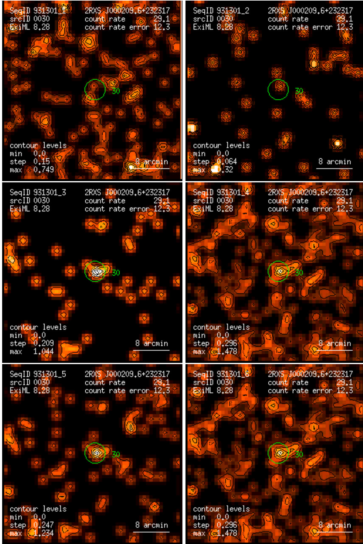
Figure 30: RASS 931301: detection 0030: band rate images, Gaussian filter: (1) PSPC channels 11 – 41, (2) 52 – 90, (3) 91 – 201, (4) 11 – 235, (5) 52 – 201, (6) 11 – 201. Broad band rates in counts/ks. Band rate contour levels in counts/ks/arcmin 2 .
