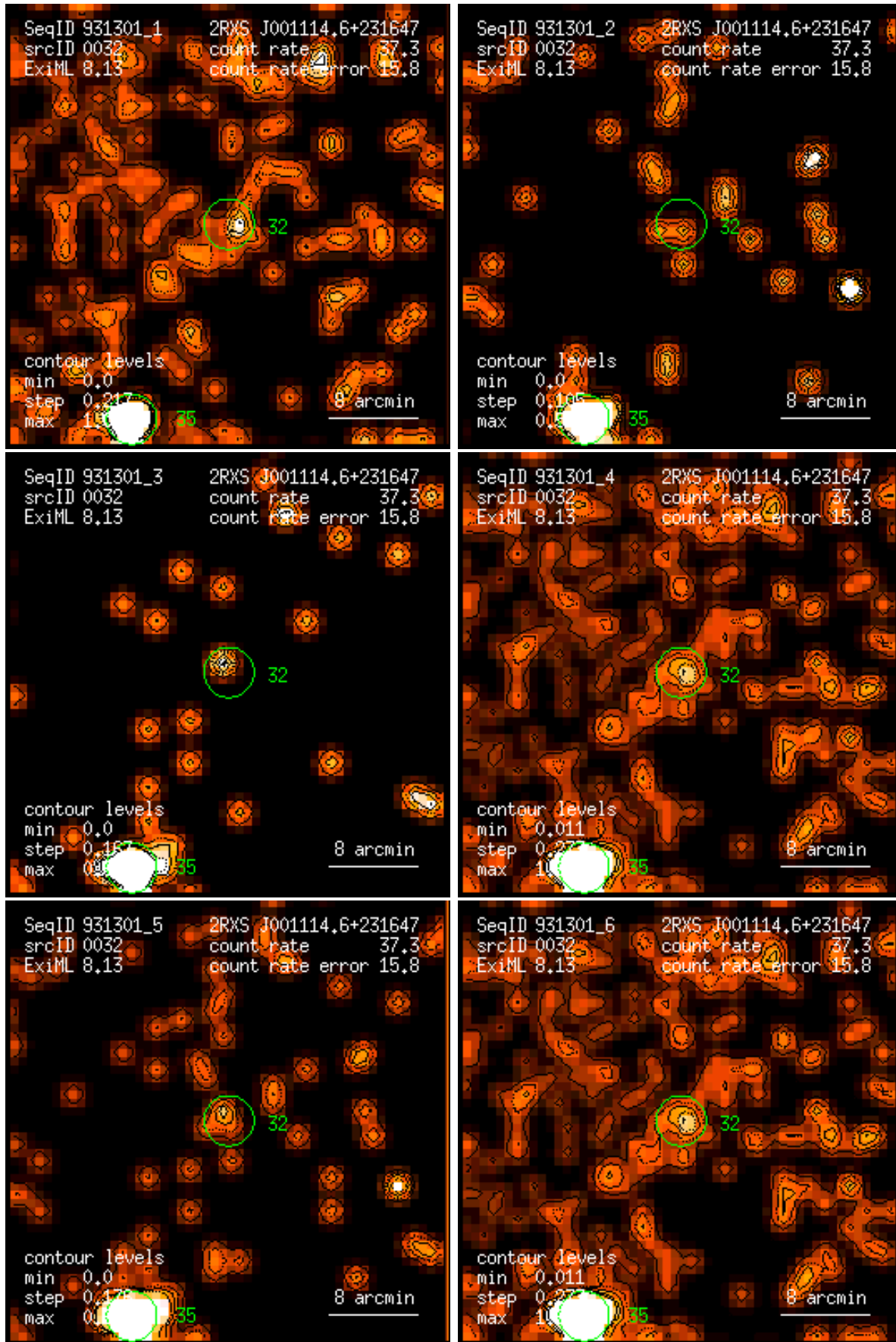
Figure 32: RASS 931301: detection 0032: band rate images, Gaussian filter: (1) PSPC channels 11 – 41, (2) 52 – 90, (3) 91 – 201, (4) 11 – 235, (5) 52 – 201, (6) 11 – 201. Broad band rates in counts/ks. Band rate contour levels in counts/ks/arcmin 2 .
