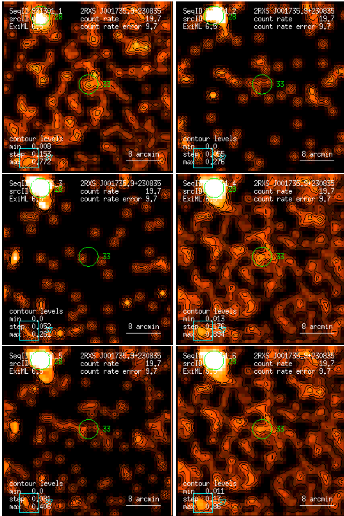
Figure 33: RASS 931301: detection 0033: band rate images, Gaussian filter: (1) PSPC channels 11 – 41, (2) 52 – 90, (3) 91 – 201, (4) 11 – 235, (5) 52 – 201, (6) 11 – 201. Broad band rates in counts/ks. Band rate contour levels in counts/ks/arcmin 2 .
