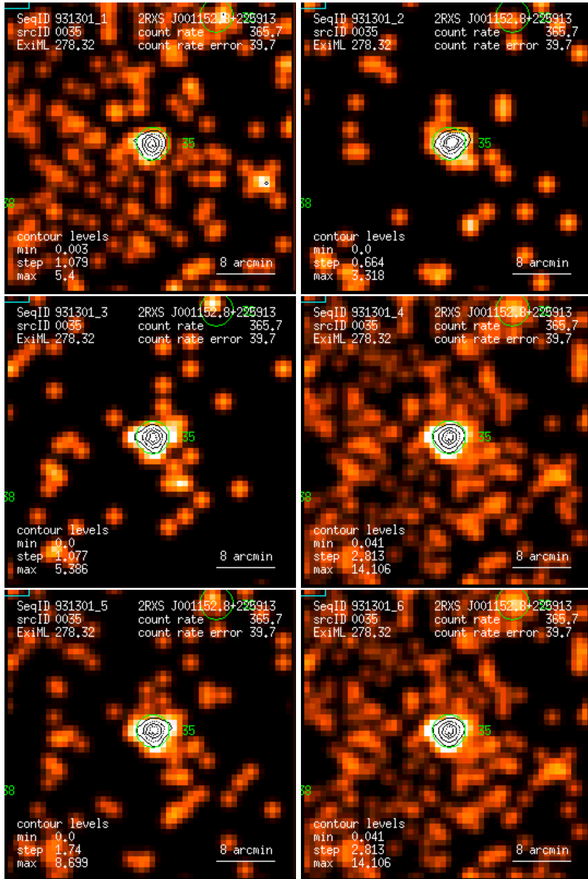
Figure 35: RASS 931301: detection 0035: band rate images, Gaussian filter: (1) PSPC channels 11 – 41, (2) 52 – 90, (3) 91 – 201, (4) 11 – 235, (5) 52 – 201, (6) 11 – 201. Broad band rates in counts/ks. Band rate contour levels in counts/ks/arcmin 2 .
