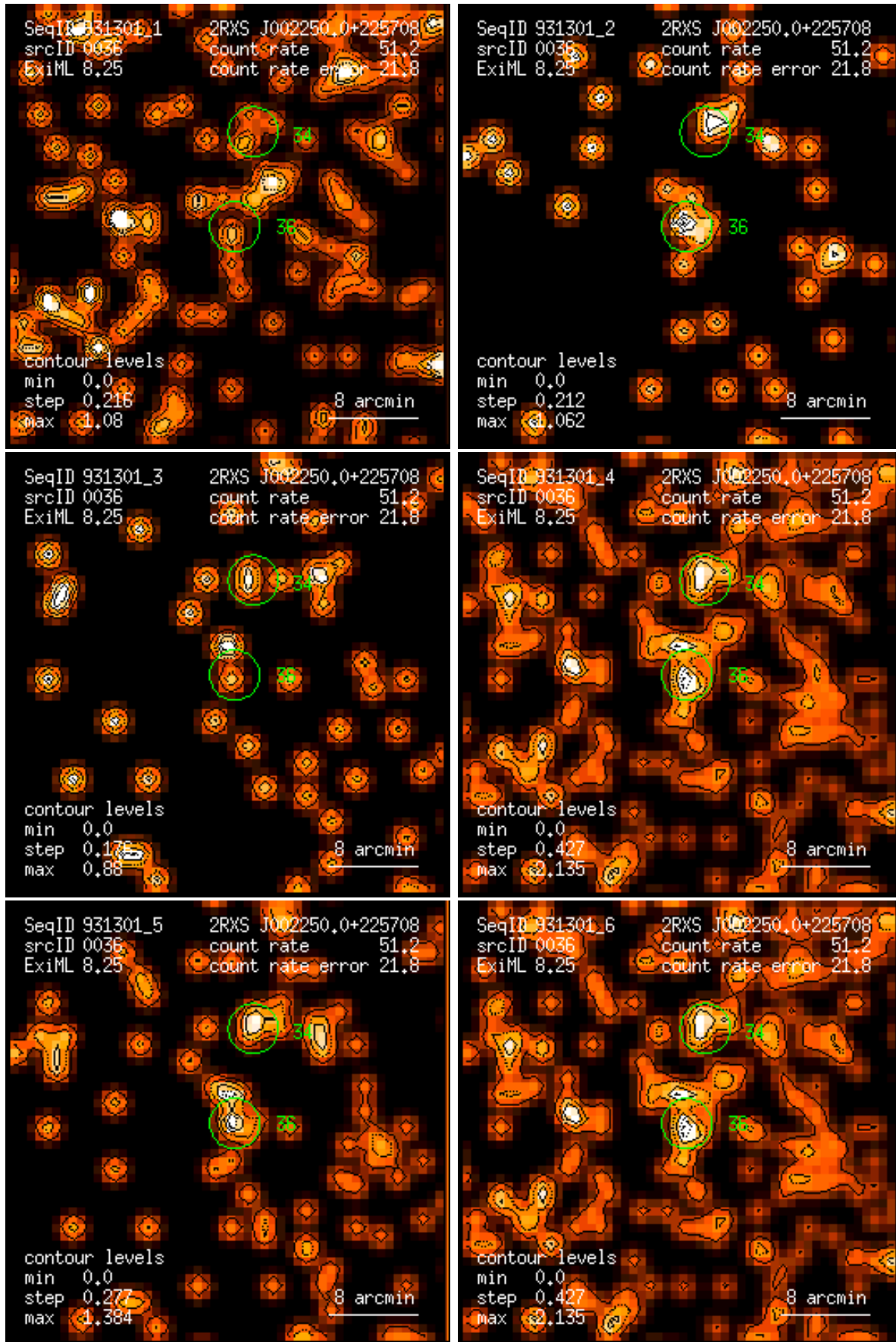
Figure 36: RASS 931301: detection 0036: band rate images, Gaussian filter: (1) PSPC channels 11 – 41, (2) 52 – 90, (3) 91 – 201, (4) 11 – 235, (5) 52 – 201, (6) 11 – 201. Broad band rates in counts/ks. Band rate contour levels in counts/ks/arcmin 2 .
