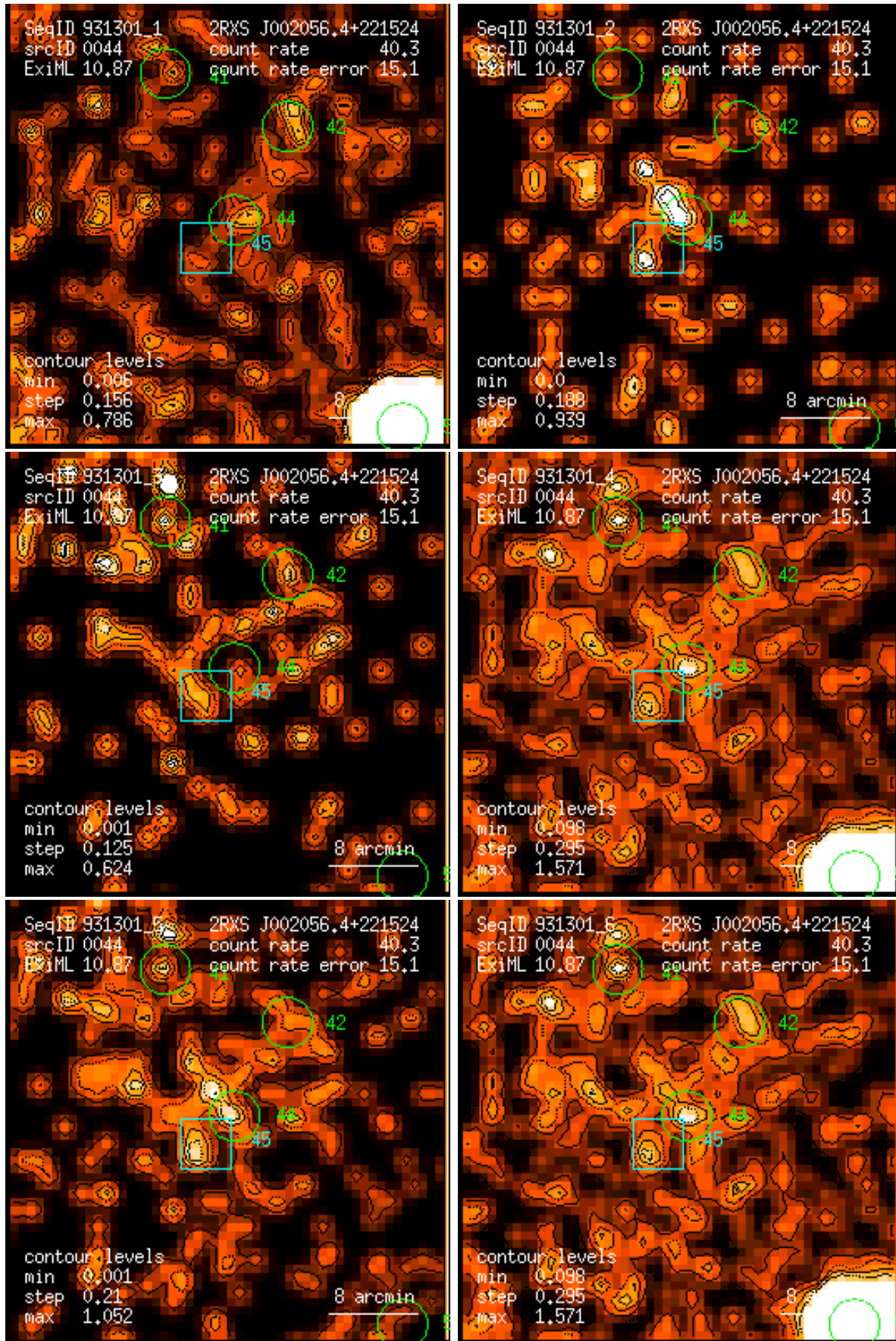
Figure 44: RASS 931301: detection 0044: band rate images, Gaussian filter: (1) PSPC channels 11 – 41, (2) 52 – 90, (3) 91 – 201, (4) 11 – 235, (5) 52 – 201, (6) 11 – 201. Broad band rates in counts/ks. Band rate contour levels in counts/ks/arcmin 2 .
