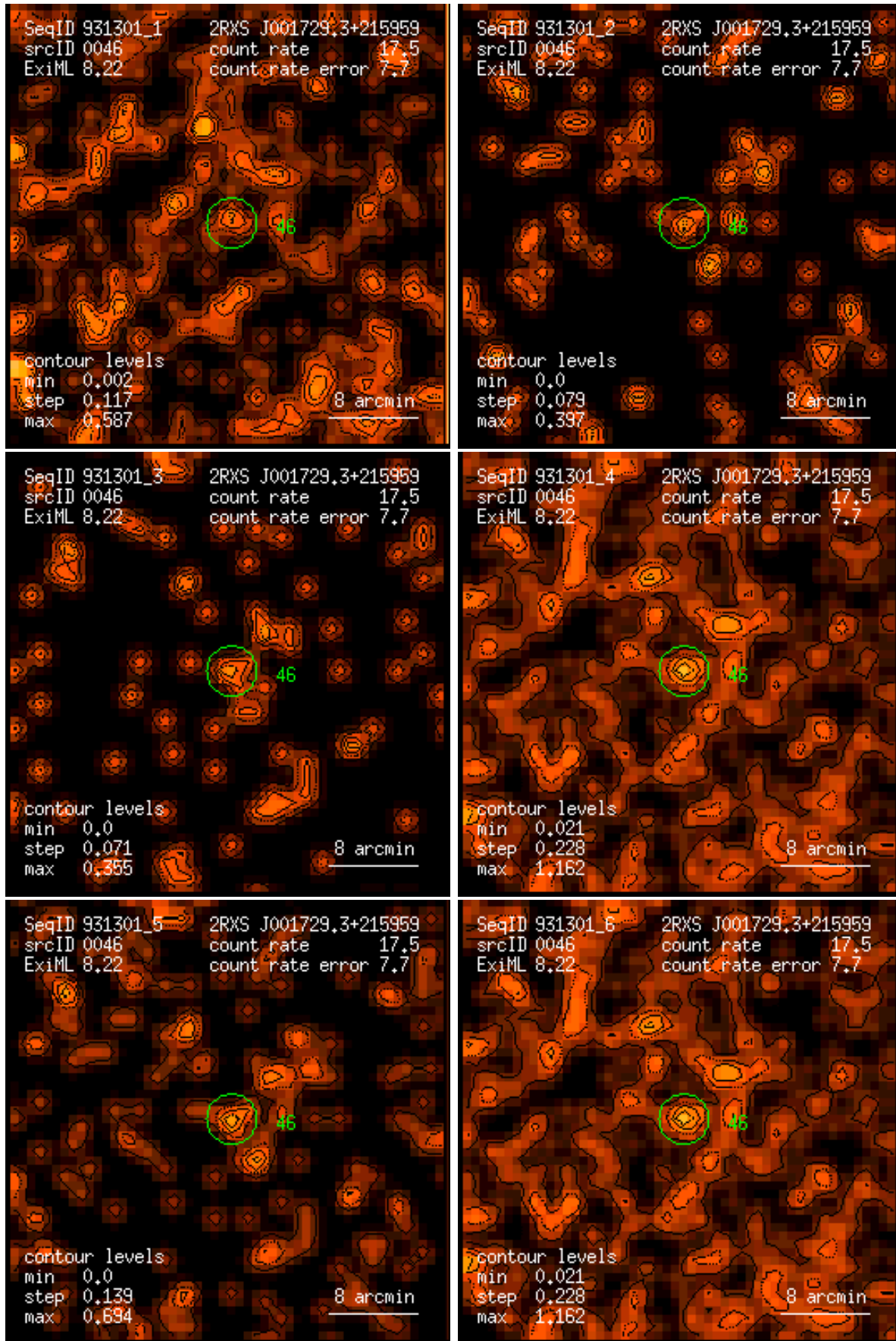
Figure 46: RASS 931301: detection 0046: band rate images, Gaussian filter: (1) PSPC channels 11 – 41, (2) 52 – 90, (3) 91 – 201, (4) 11 – 235, (5) 52 – 201, (6) 11 – 201. Broad band rates in counts/ks. Band rate contour levels in counts/ks/arcmin 2 .
