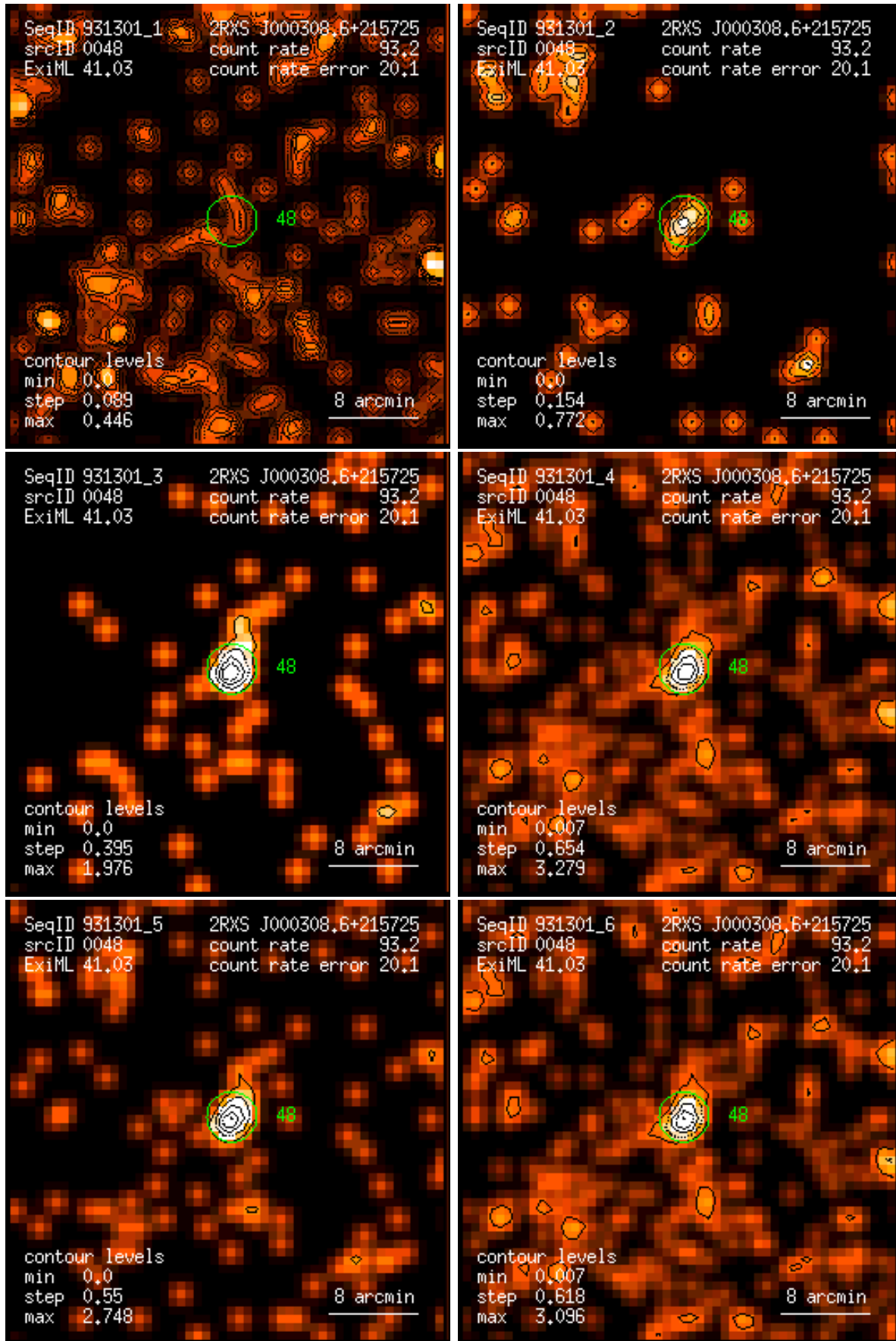
Figure 48: RASS 931301: detection 0048: band rate images, Gaussian filter: (1) PSPC channels 11 – 41, (2) 52 – 90, (3) 91 – 201, (4) 11 – 235, (5) 52 – 201, (6) 11 – 201. Broad band rates in counts/ks. Band rate contour levels in counts/ks/arcmin 2 .
