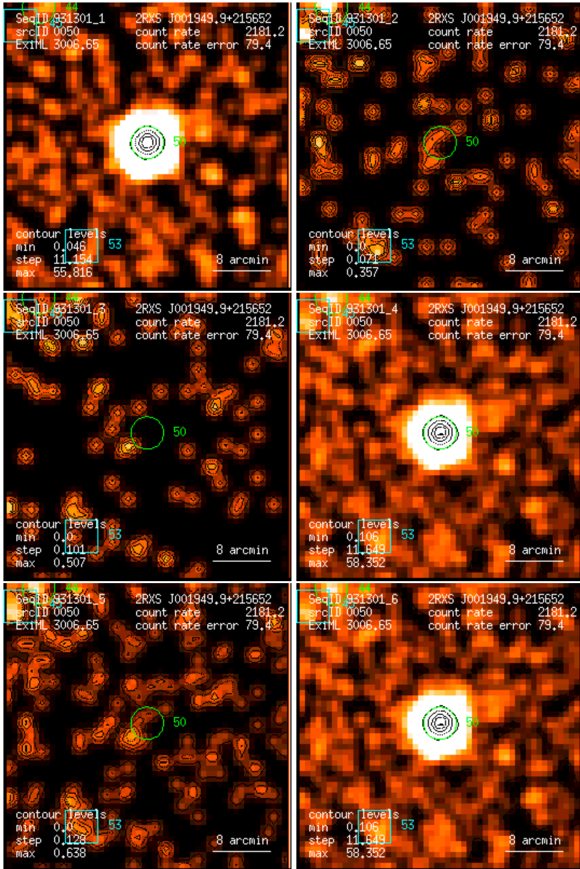
Figure 50: RASS 931301: detection 0050: band rate images, Gaussian filter: (1) PSPC channels 11 – 41, (2) 52 – 90, (3) 91 – 201, (4) 11 – 235, (5) 52 – 201, (6) 11 – 201. Broad band rates in counts/ks. Band rate contour levels in counts/ks/arcmin 2 .
