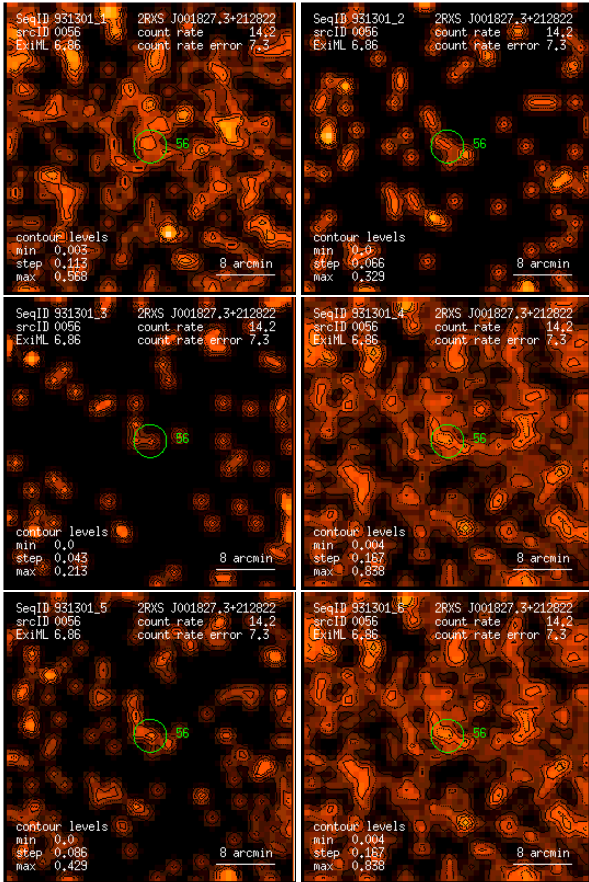
Figure 56: RASS 931301: detection 0056: band rate images, Gaussian filter: (1) PSPC channels 11 – 41, (2) 52 – 90, (3) 91 – 201, (4) 11 – 235, (5) 52 – 201, (6) 11 – 201. Broad band rates in counts/ks. Band rate contour levels in counts/ks/arcmin 2 .
