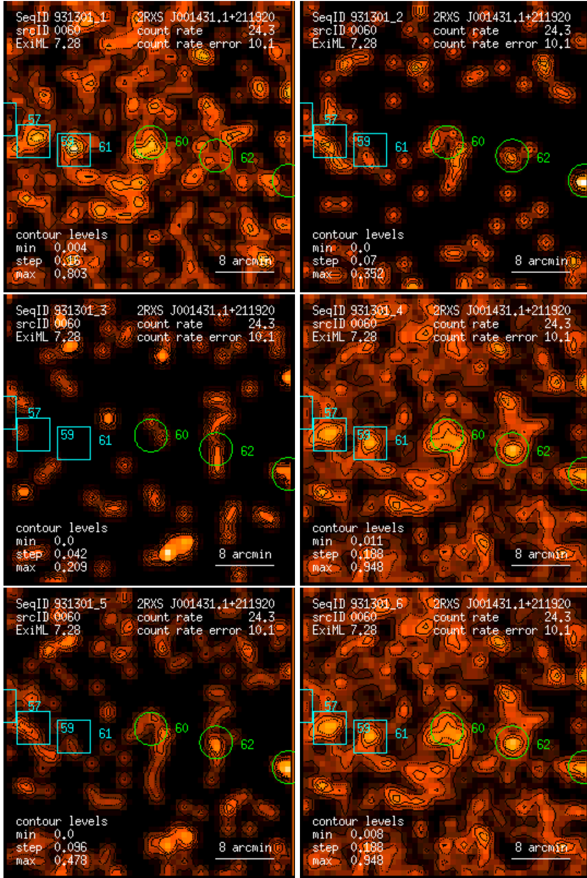
Figure 60: RASS 931301: detection 0060: band rate images, Gaussian filter: (1) PSPC channels 11 – 41, (2) 52 – 90, (3) 91 – 201, (4) 11 – 235, (5) 52 – 201, (6) 11 – 201. Broad band rates in counts/ks. Band rate contour levels in counts/ks/arcmin 2 .
